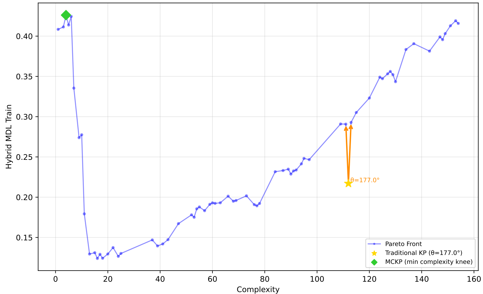
556_analcatdata_apnea2 - Run 26 - MVP - Hybrid MDL Train \lambda_1=0.00 , \lambda_2=0.00 , \lambda_3=0.00 | Difficulty: 1.00 | Method: hmr
