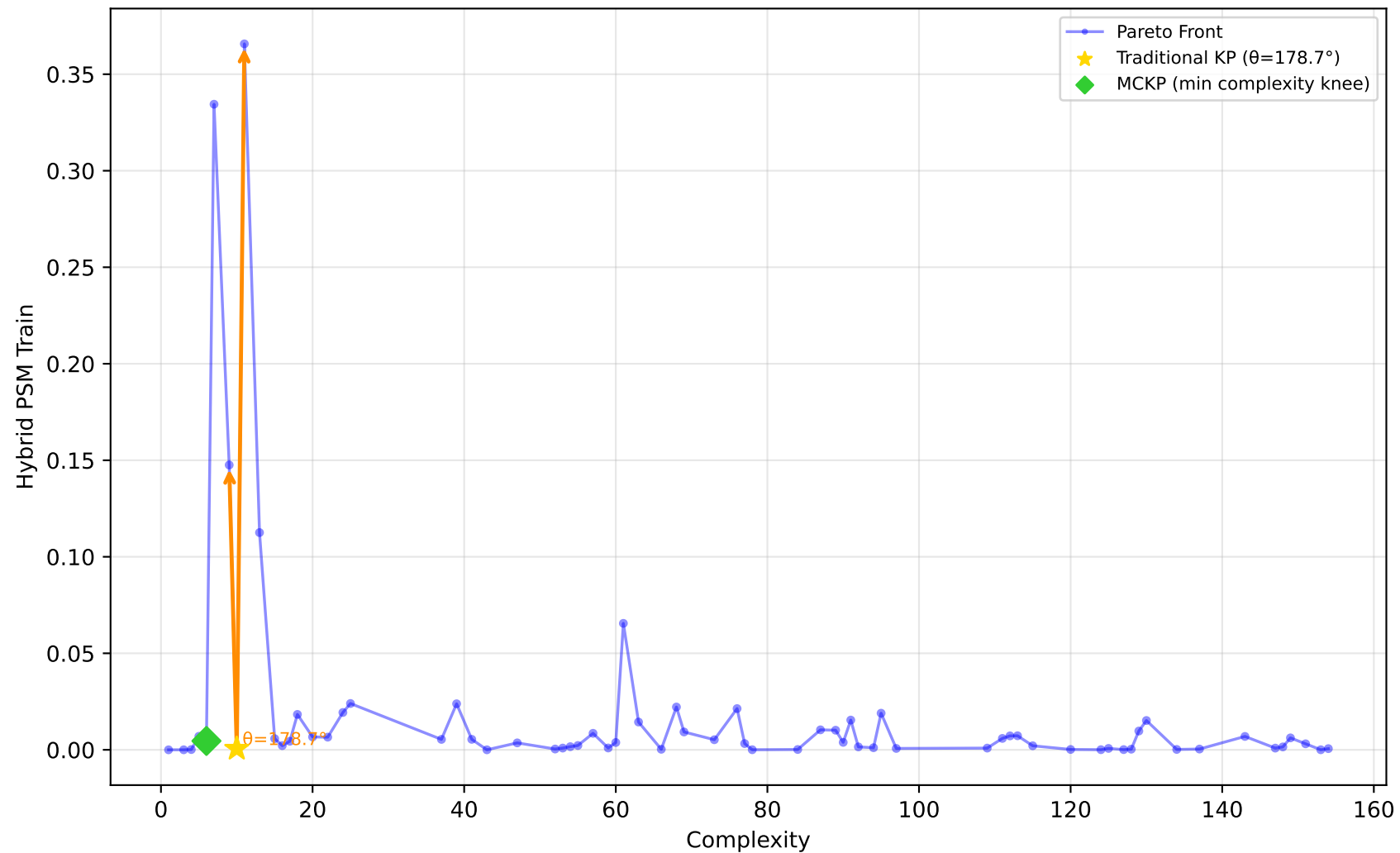
556_analcatdata_apnea2 - Run 26 - MVP - Hybrid PSM Train \lambda_1=0.00 , \lambda_2=0.00 , \lambda_3=0.00 | Difficulty: 1.00 | Method: hmr
