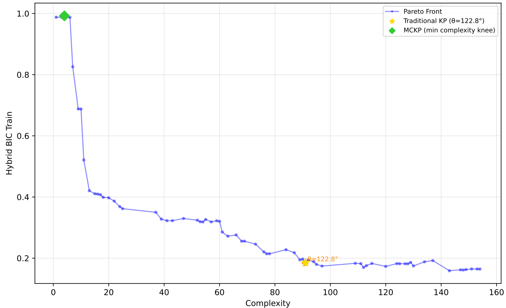
556_analcatdata_apnea2 - Run 26 - SVP - Hybrid BIC Train \lambda_1=0.00, \lambda_2=0.00, \lambda_3=0.00 | Difficulty: 1.00 | Method: hmr
