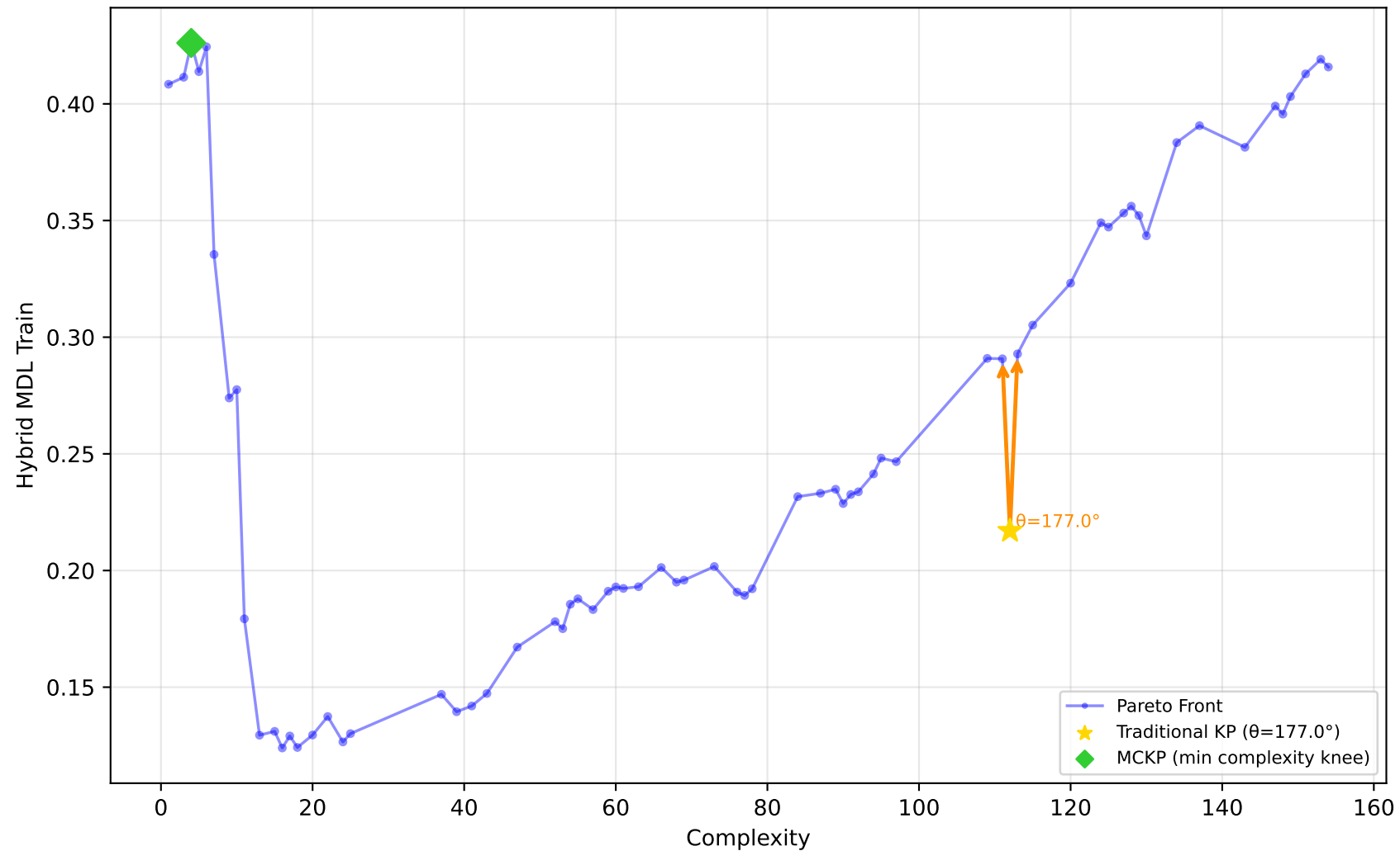
556_analcatdata_apnea2 - Run 26 - SVP - Hybrid MDL Train \lambda_1=0.00 , \lambda_2=0.00 , \lambda_3=0.00 | Difficulty: 1.00 | Method: hmr
