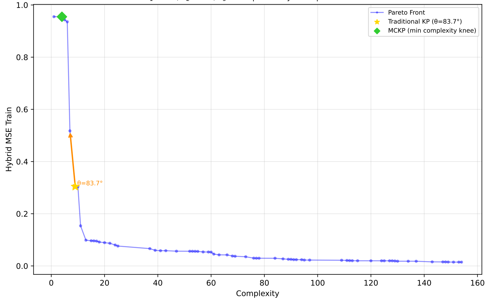
556_analcatdata_apnea2 - Run 26 - SVP - Hybrid MSE Train \lambda_1=0.00, \lambda_2=0.00, \lambda_3=0.00 | Difficulty: 1.00 | Method: hmr
