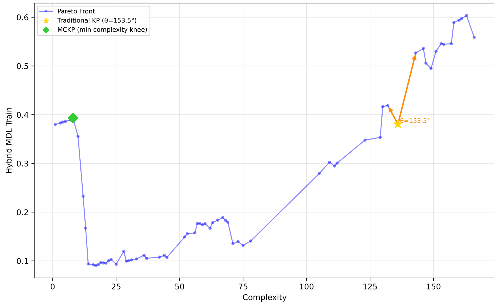
556_analcatdata_apnea2 - Run 27 - MVP - Hybrid MDL Train \lambda_1=0.00, \lambda_2=0.00, \lambda_3=0.00 | Difficulty: 1.00 | Method: hmr
