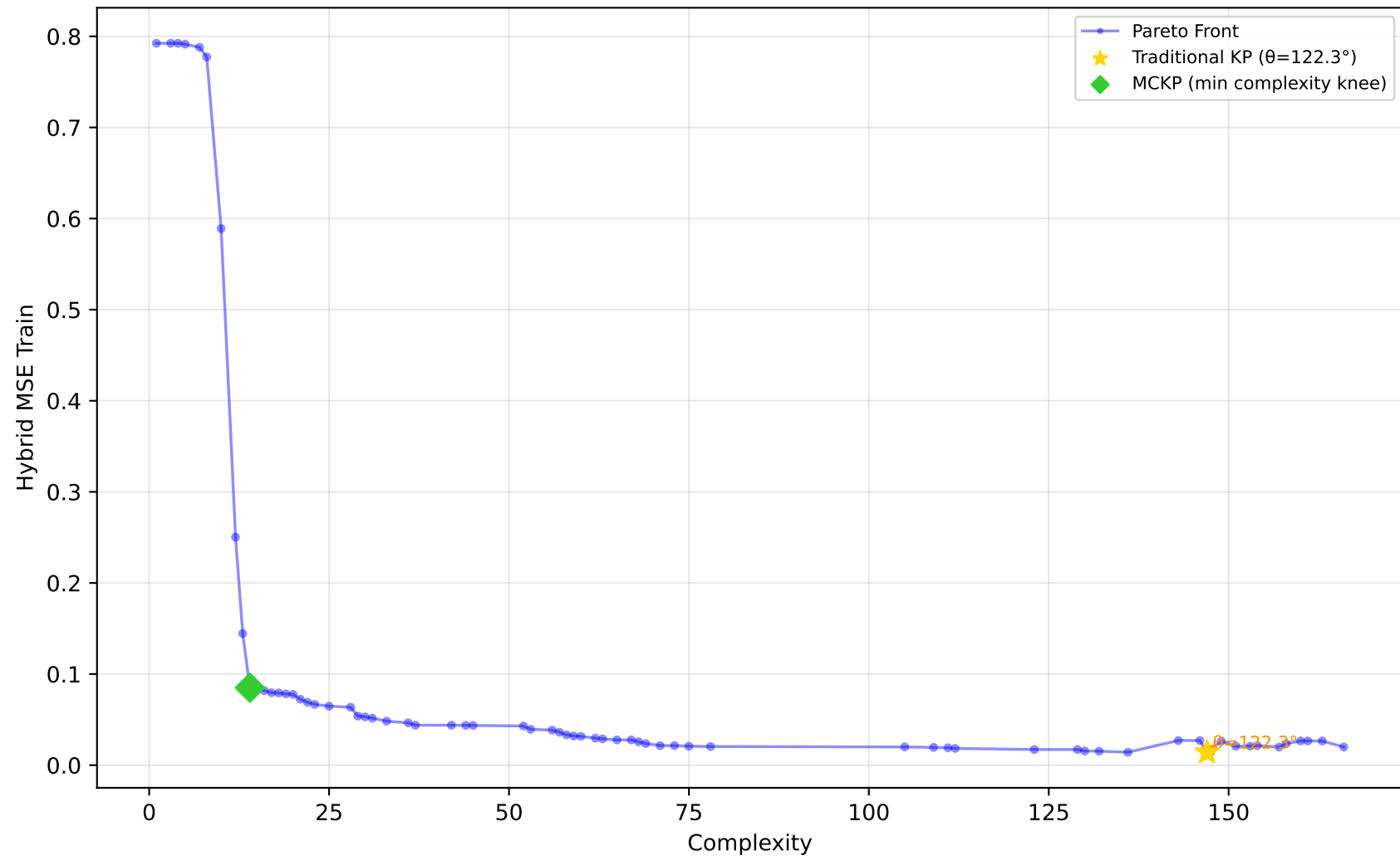
556_analcatdata_apnea2 - Run 27 - SVP - Hybrid MSE Train \lambda_1=0.00, \lambda_2=0.00, \lambda_3=0.00 | Difficulty: 1.00 | Method: hmr
