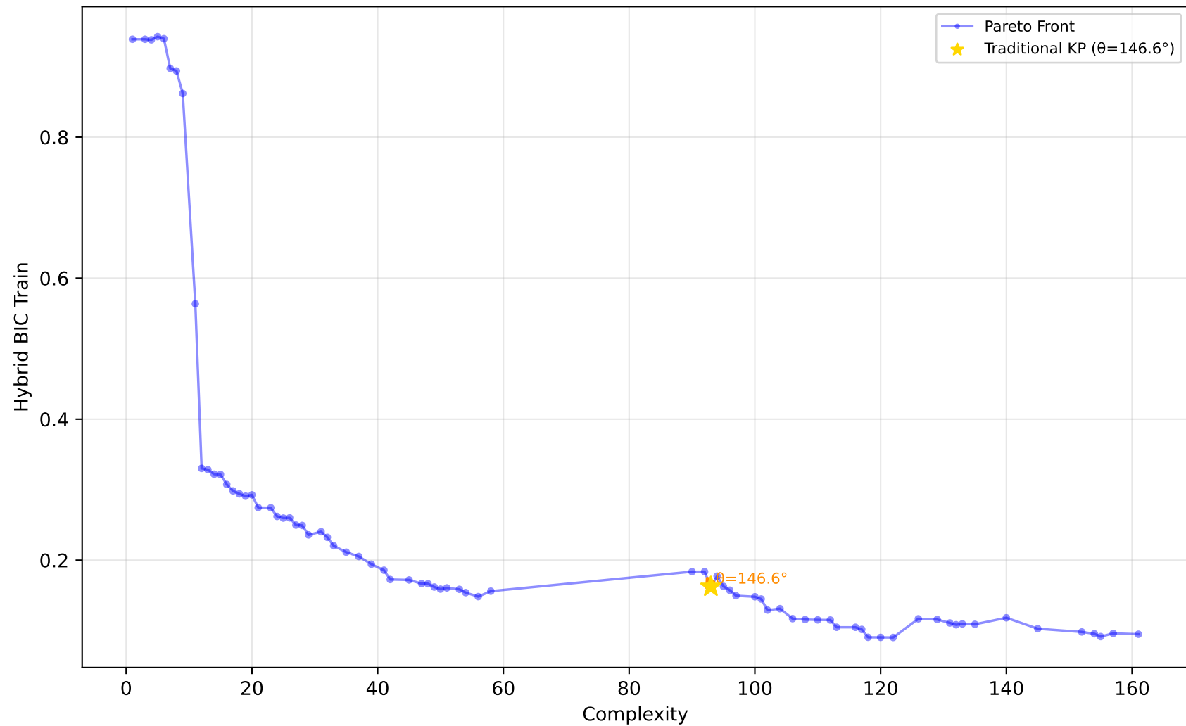
556_analcatdata_apnea2 - Run 28 - MVP - Hybrid BIC Train \lambda_1=0.00, \lambda_2=0.00, \lambda_3=0.00 | Difficulty: 1.00 | Method: hmr
