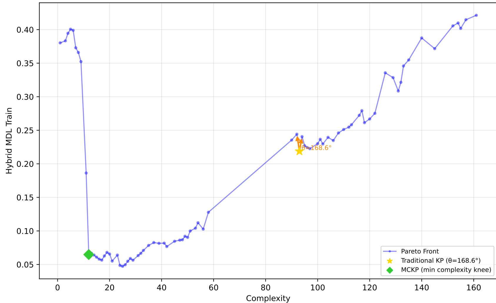
556_analcatdata_apnea2 - Run 28 - MVP - Hybrid MDL Train \lambda_1=0.00 , \lambda_2=0.00 , \lambda_3=0.00 | Difficulty: 1.00 | Method: hmr
