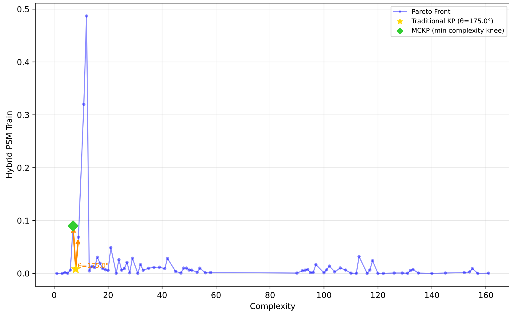
556_analcatdata_apnea2 - Run 28 - MVP - Hybrid PSM Train \lambda_1=0.00, \lambda_2=0.00, \lambda_3=0.00 | Difficulty: 1.00 | Method: hmr
