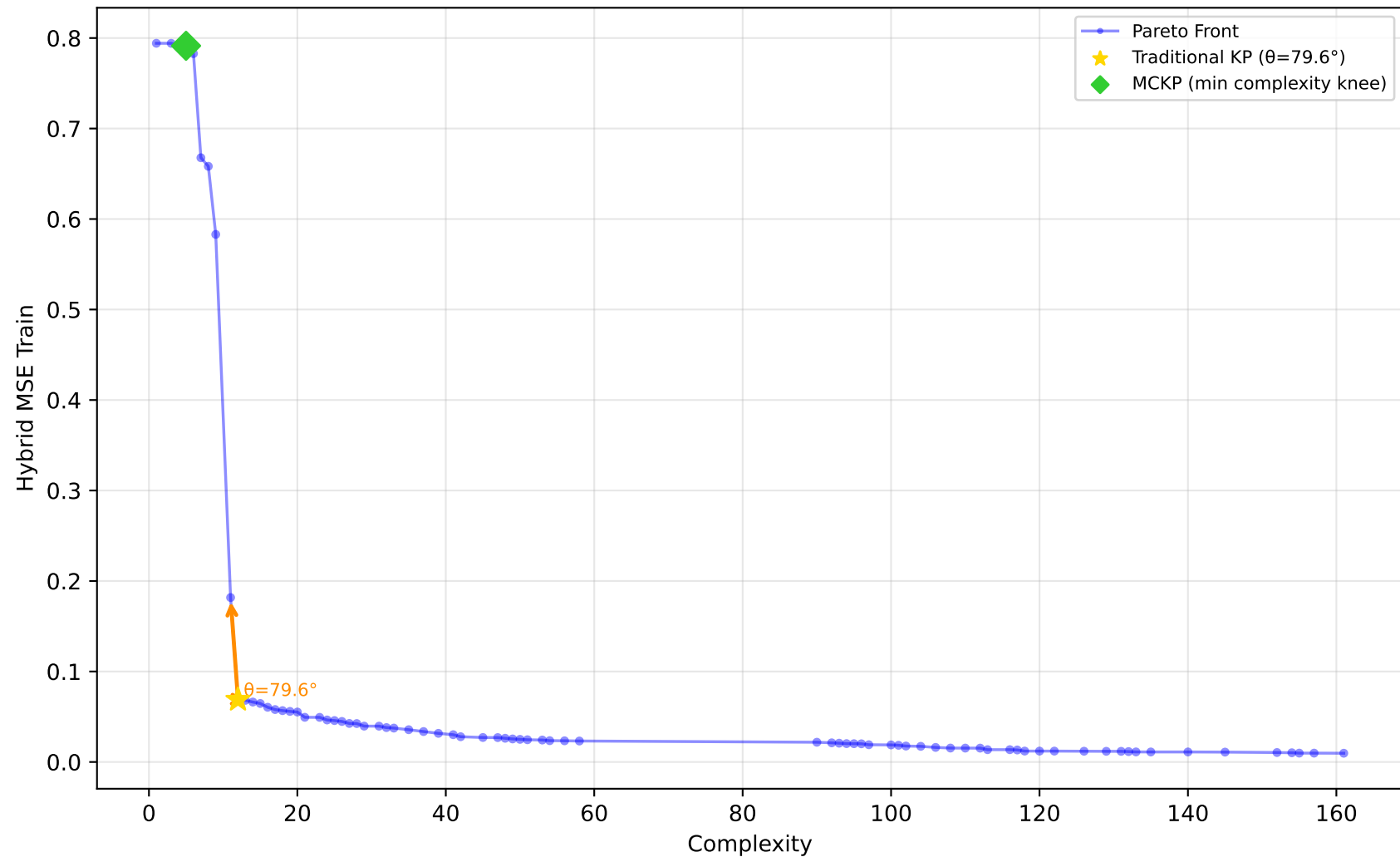
556_analcatdata_apnea2 - Run 28 - SVP - Hybrid MSE Train \lambda_1=0.00, \lambda_2=0.00, \lambda_3=0.00 | Difficulty: 1.00 | Method: hmr
