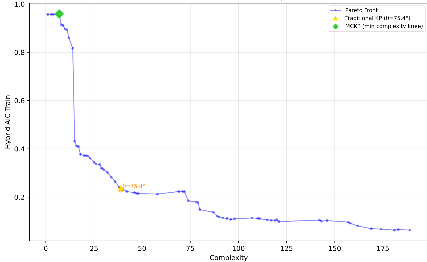
556_analcatdata_apnea2 - Run 29 - SVP - Hybrid AIC Train \lambda_1=0.00, \lambda_2=0.00, \lambda_3=0.00 | Difficulty: 1.00 | Method: hmr
