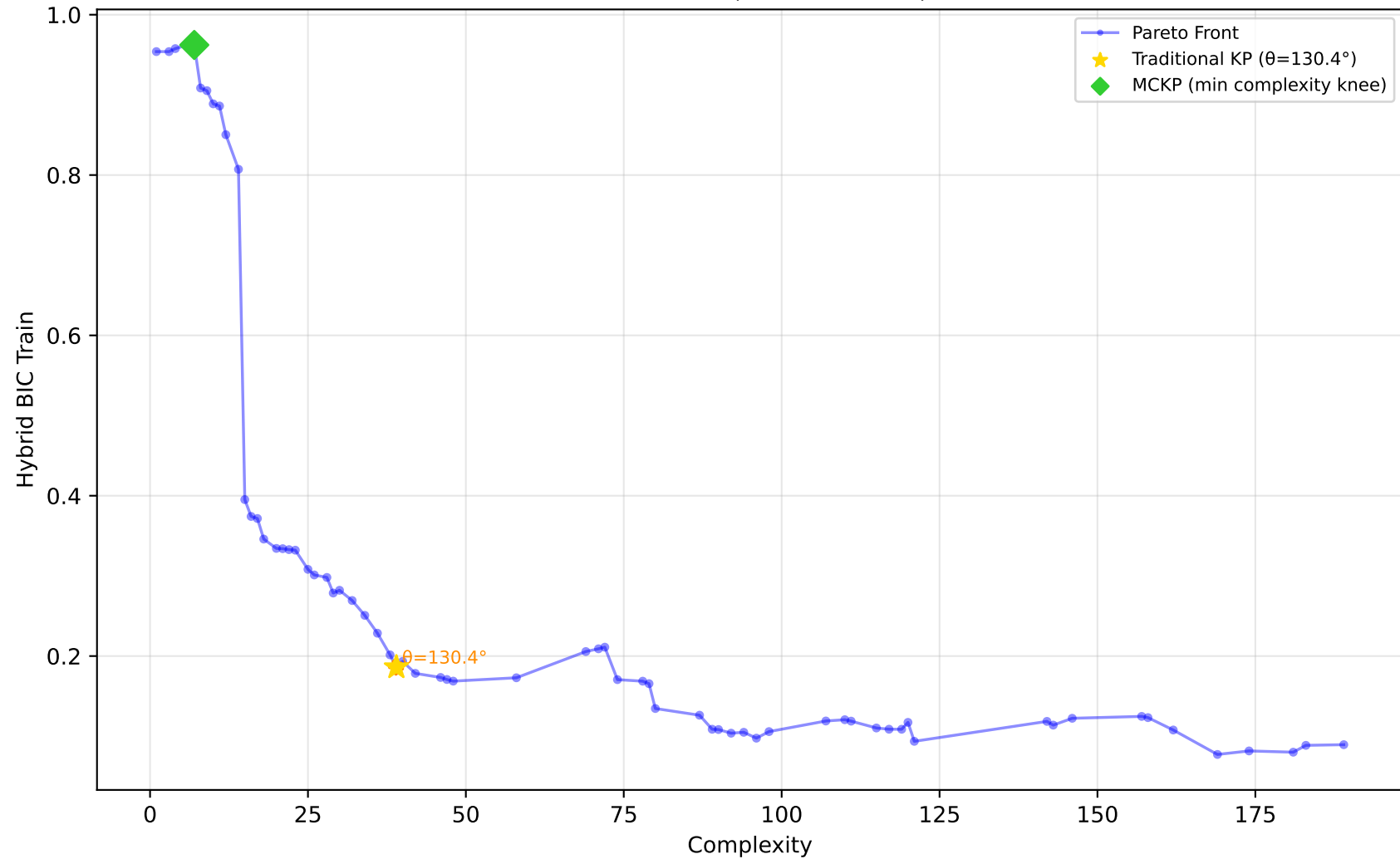
556_analcatdata_apnea2 - Run 29 - SVP - Hybrid BIC Train \lambda_1=0.00 , \lambda_2=0.00 , \lambda_3=0.00 | Difficulty: 1.00 | Method: hmr
