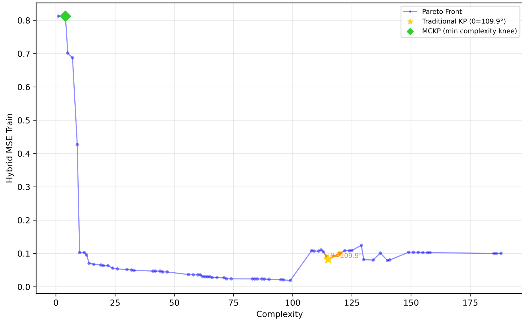
556_analcatdata_apnea2 - Run 2 - MVP - Hybrid MSE Train \lambda_1=0.00, \lambda_2=0.00, \lambda_3=0.00 | Difficulty: 1.00 | Method: hmr
