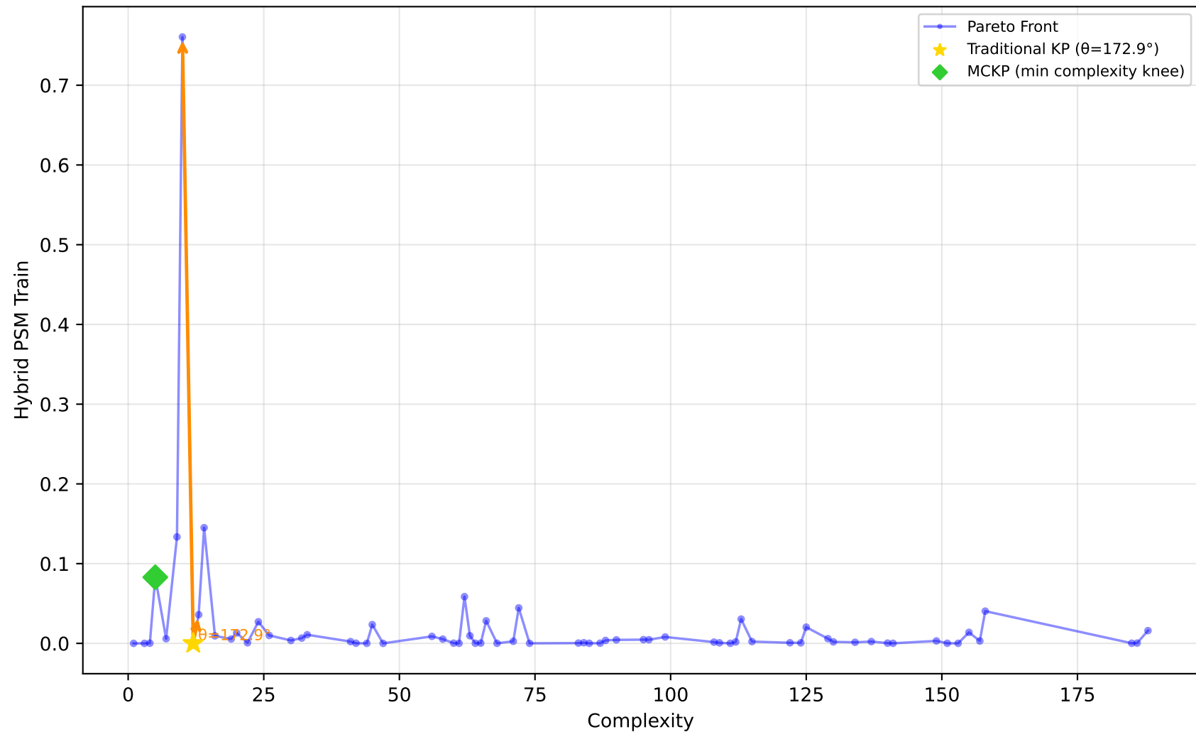
556_analcatdata_apnea2 - Run 2 - MVP - Hybrid PSM Train \lambda_1=0.00, \lambda_2=0.00, \lambda_3=0.00 | Difficulty: 1.00 | Method: hmr
