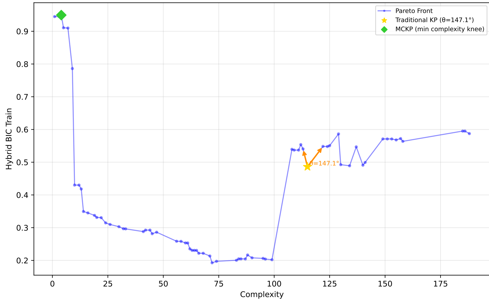
556_analcatdata_apnea2 - Run 2 - SVP - Hybrid BIC Train \lambda_1=0.00, \lambda_2=0.00, \lambda_3=0.00 | Difficulty: 1.00 | Method: hmr
