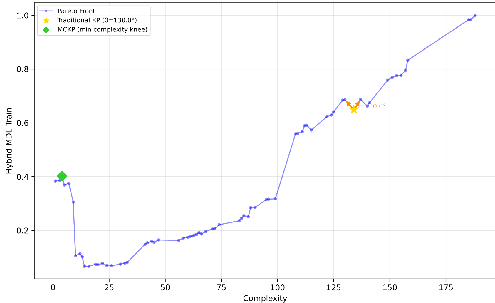
556_analcatdata_apnea2 - Run 2 - SVP - Hybrid MDL Train \lambda_1=0.00, \lambda_2=0.00, \lambda_3=0.00 | Difficulty: 1.00 | Method: hmr
