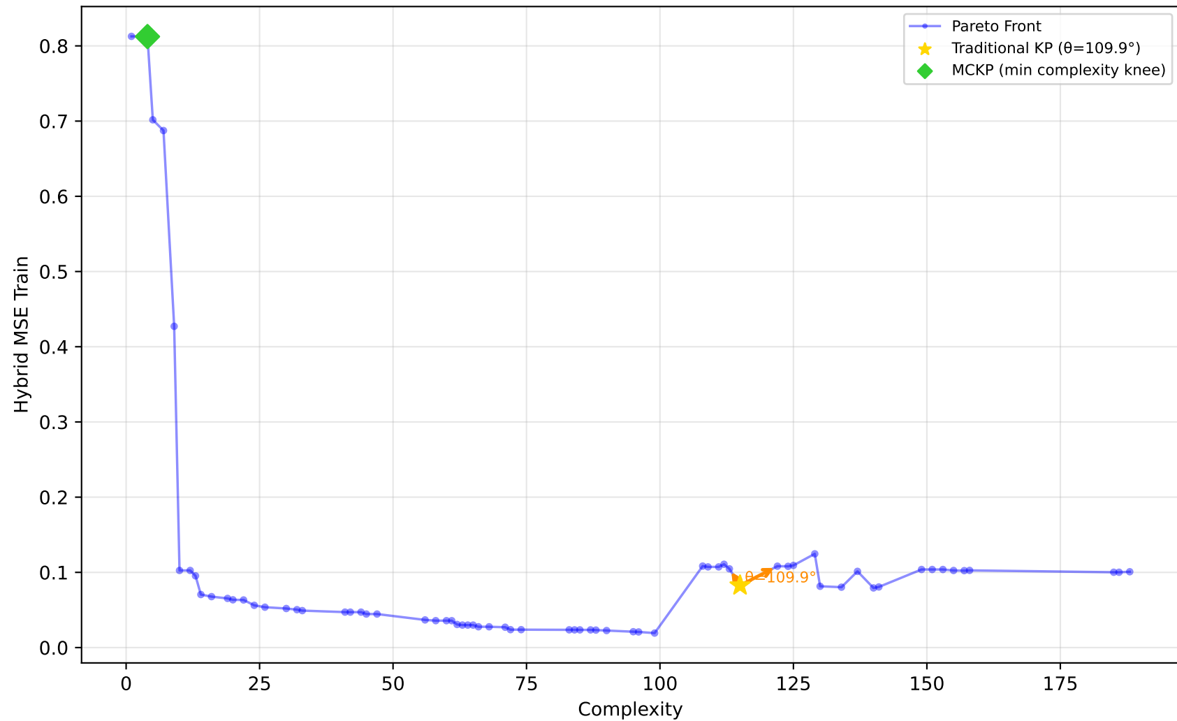
556_analcatdata_apnea2 - Run 2 - SVP - Hybrid MSE Train \lambda_1=0.00, \lambda_2=0.00, \lambda_3=0.00 | Difficulty: 1.00 | Method: hmr
