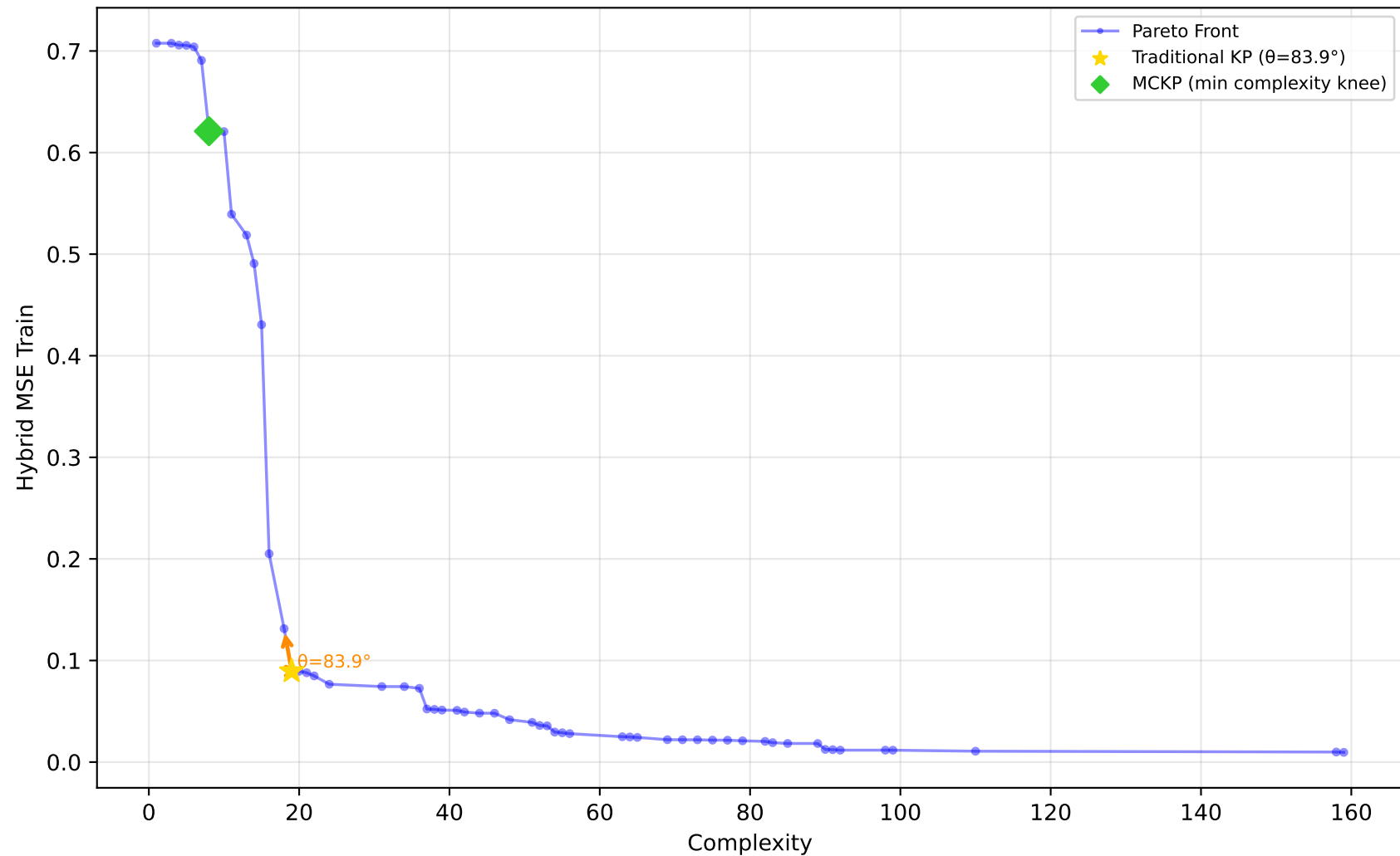
556_analcatdata_apnea2 - Run 30 - MVP - Hybrid MSE Train \lambda_1=0.00, \lambda_2=0.00, \lambda_3=0.00 | Difficulty: 1.00 | Method: hmr
