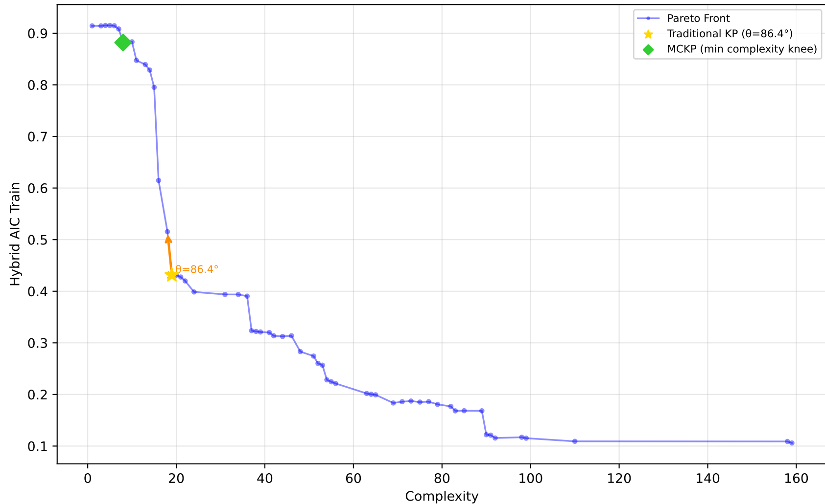
556_analcatdata_apnea2 - Run 30 - SVP - Hybrid AIC Train \lambda_1=0.00, \lambda_2=0.00, \lambda_3=0.00 | Difficulty: 1.00 | Method: hmr
