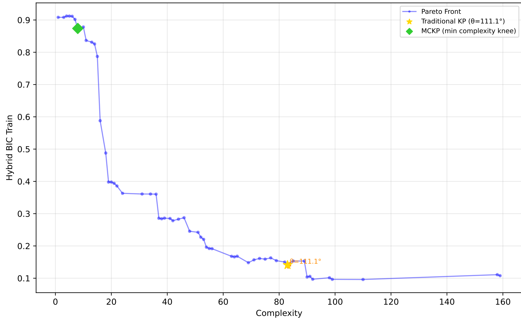
556_analcatdata_apnea2 - Run 30 - SVP - Hybrid BIC Train \lambda_1=0.00, \lambda_2=0.00, \lambda_3=0.00 | Difficulty: 1.00 | Method: hmr
