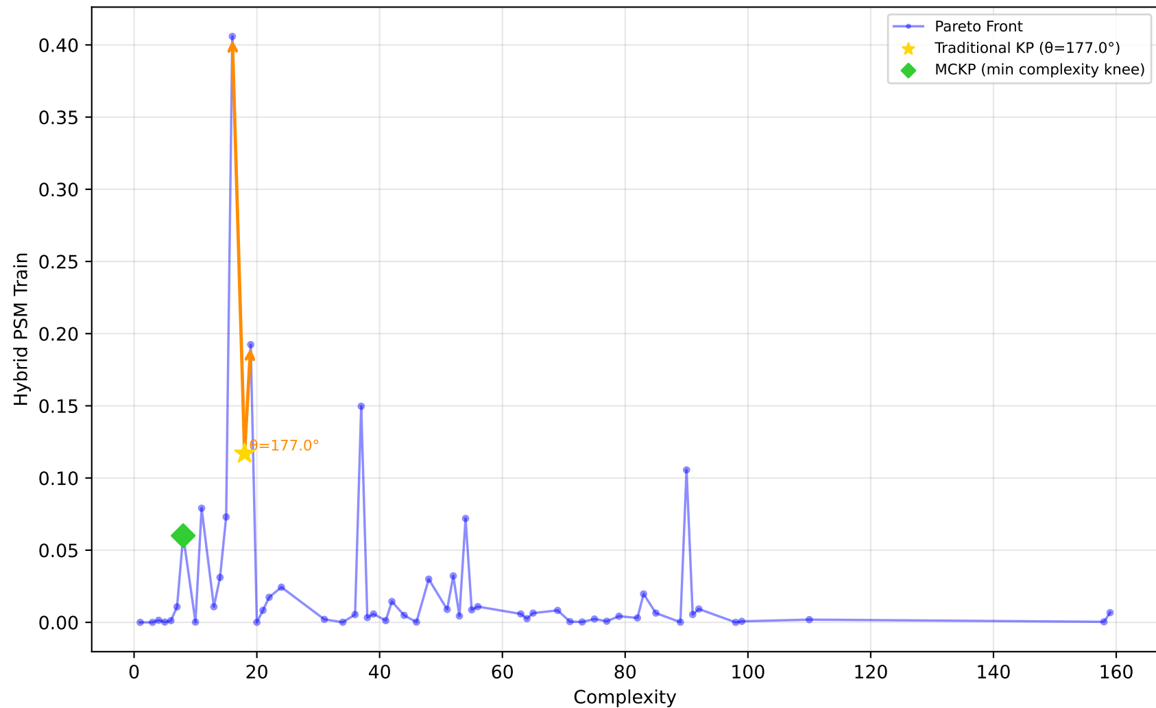
556_analcatdata_apnea2 - Run 30 - SVP - Hybrid PSM Train \lambda_1=0.00 , \lambda_2=0.00 , \lambda_3=0.00 | Difficulty: 1.00 | Method: hmr
