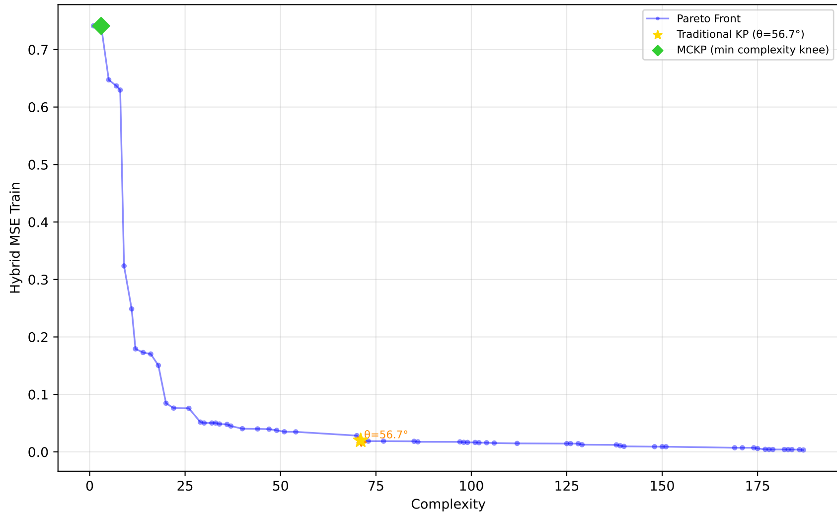
556_analcatdata_apnea2 - Run 3 - MVP - Hybrid MSE Train \lambda_1=0.00, \lambda_2=0.00, \lambda_3=0.00 | Difficulty: 1.00 | Method: hmr
