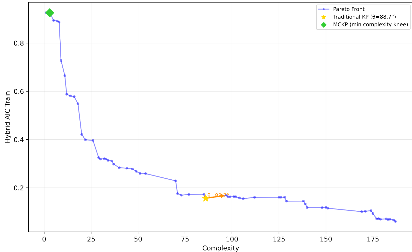
556_analcatdata_apnea2 - Run 3 - SVP - Hybrid AIC Train \lambda_1=0.00, \lambda_2=0.00, \lambda_3=0.00 | Difficulty: 1.00 | Method: hmr
