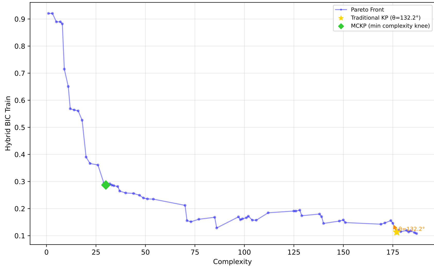
556_analcatdata_apnea2 - Run 3 - SVP - Hybrid BIC Train \lambda_1=0.00, \lambda_2=0.00, \lambda_3=0.00 | Difficulty: 1.00 | Method: hmr
