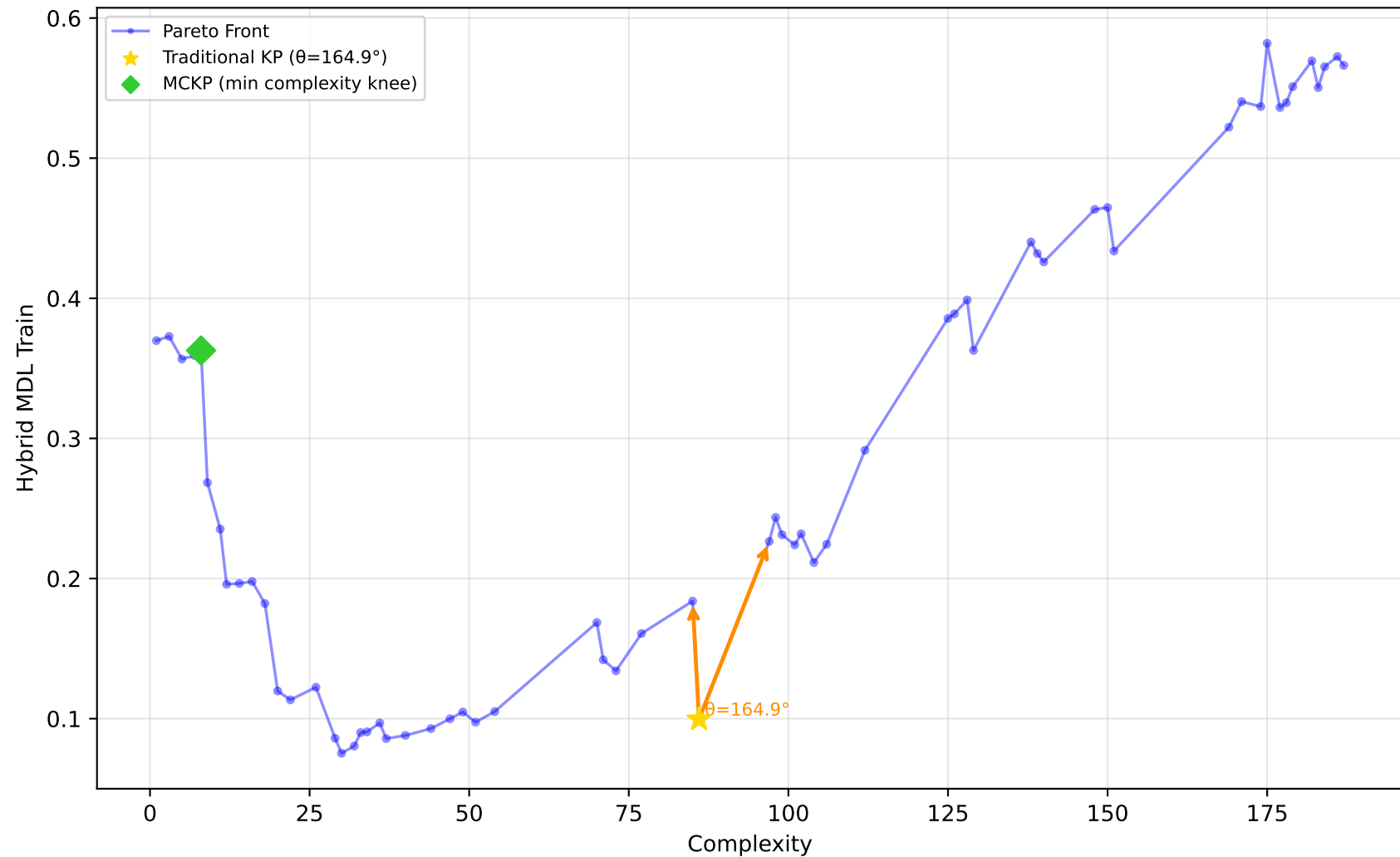
556_analcatdata_apnea2 - Run 3 - SVP - Hybrid MDL Train \lambda_1=0.00 , \lambda_2=0.00 , \lambda_3=0.00 | Difficulty: 1.00 | Method: hmr
