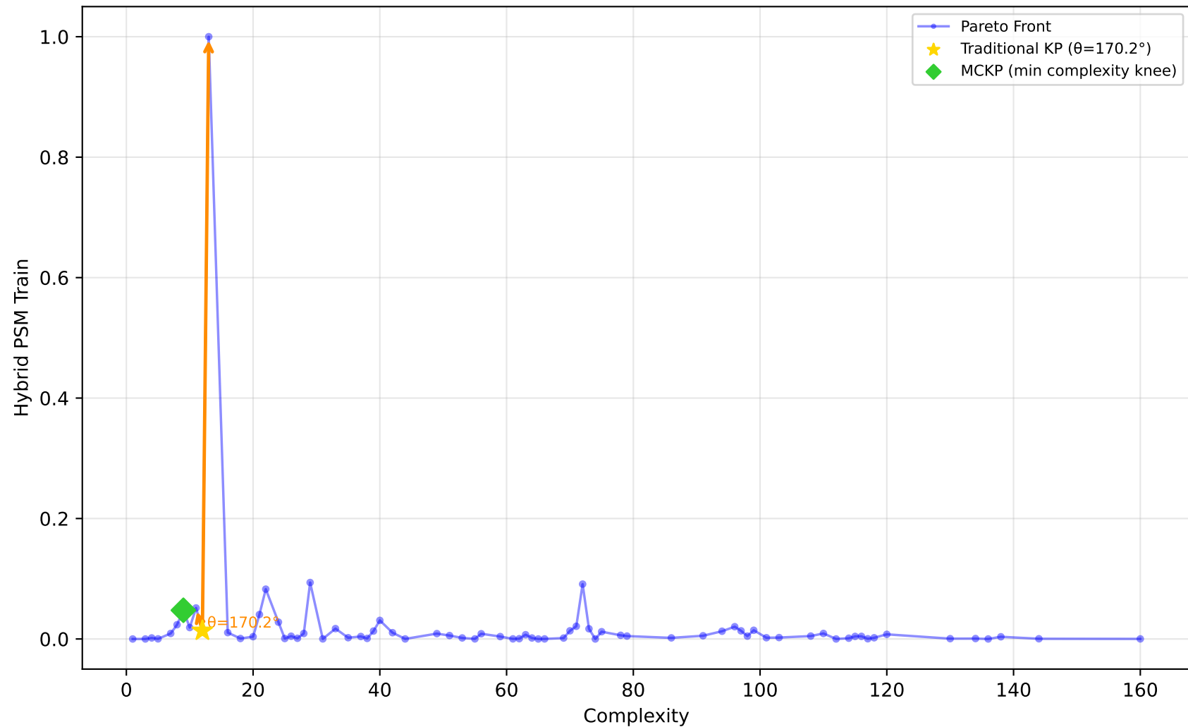
556_analcatdata_apnea2 - Run 4 - MVP - Hybrid PSM Train \lambda_1=0.00, \lambda_2=0.00, \lambda_3=0.00 | Difficulty: 1.00 | Method: hmr
