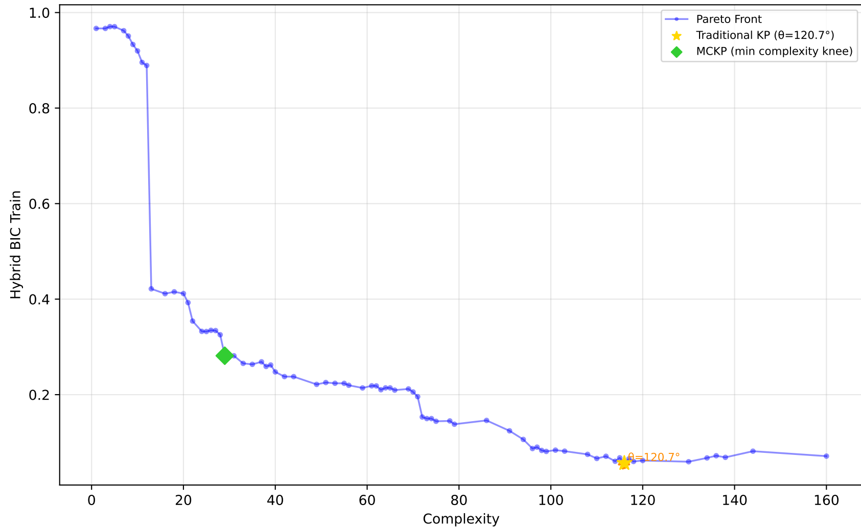
556_analcatdata_apnea2 - Run 4 - SVP - Hybrid BIC Train \lambda_1=0.00, \lambda_2=0.00, \lambda_3=0.00 | Difficulty: 1.00 | Method: hmr
