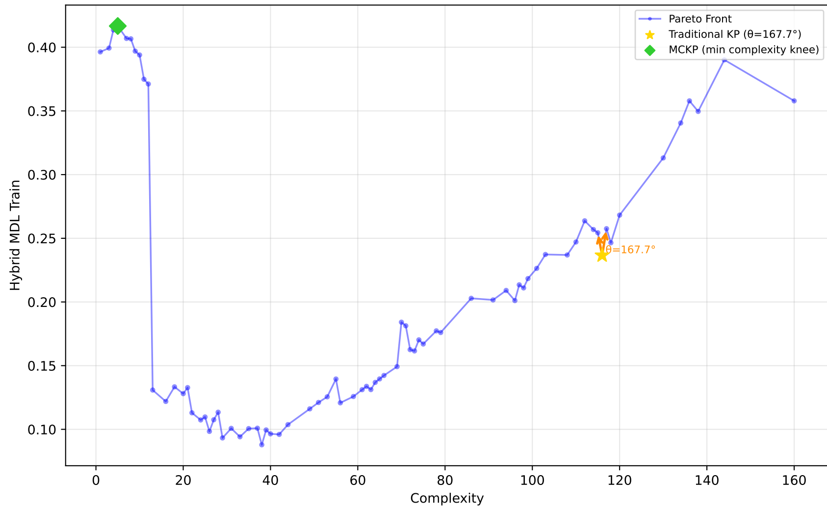
556_analcatdata_apnea2 - Run 4 - SVP - Hybrid MDL Train \lambda_1=0.00, \lambda_2=0.00, \lambda_3=0.00 | Difficulty: 1.00 | Method: hmr
