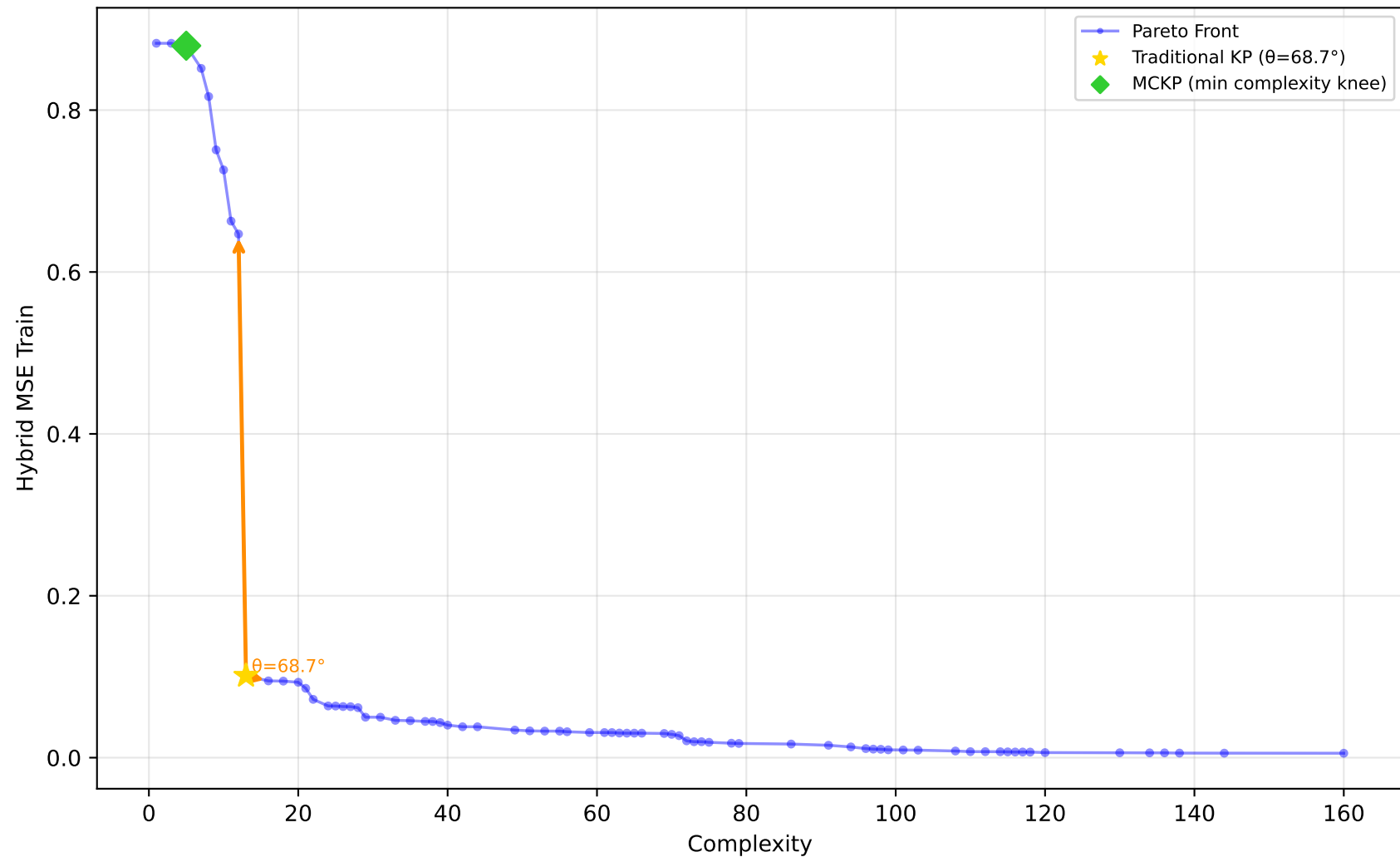
556_analcatdata_apnea2 - Run 4 - SVP - Hybrid MSE Train \lambda_1=0.00 , \lambda_2=0.00 , \lambda_3=0.00 | Difficulty: 1.00 | Method: hmr
