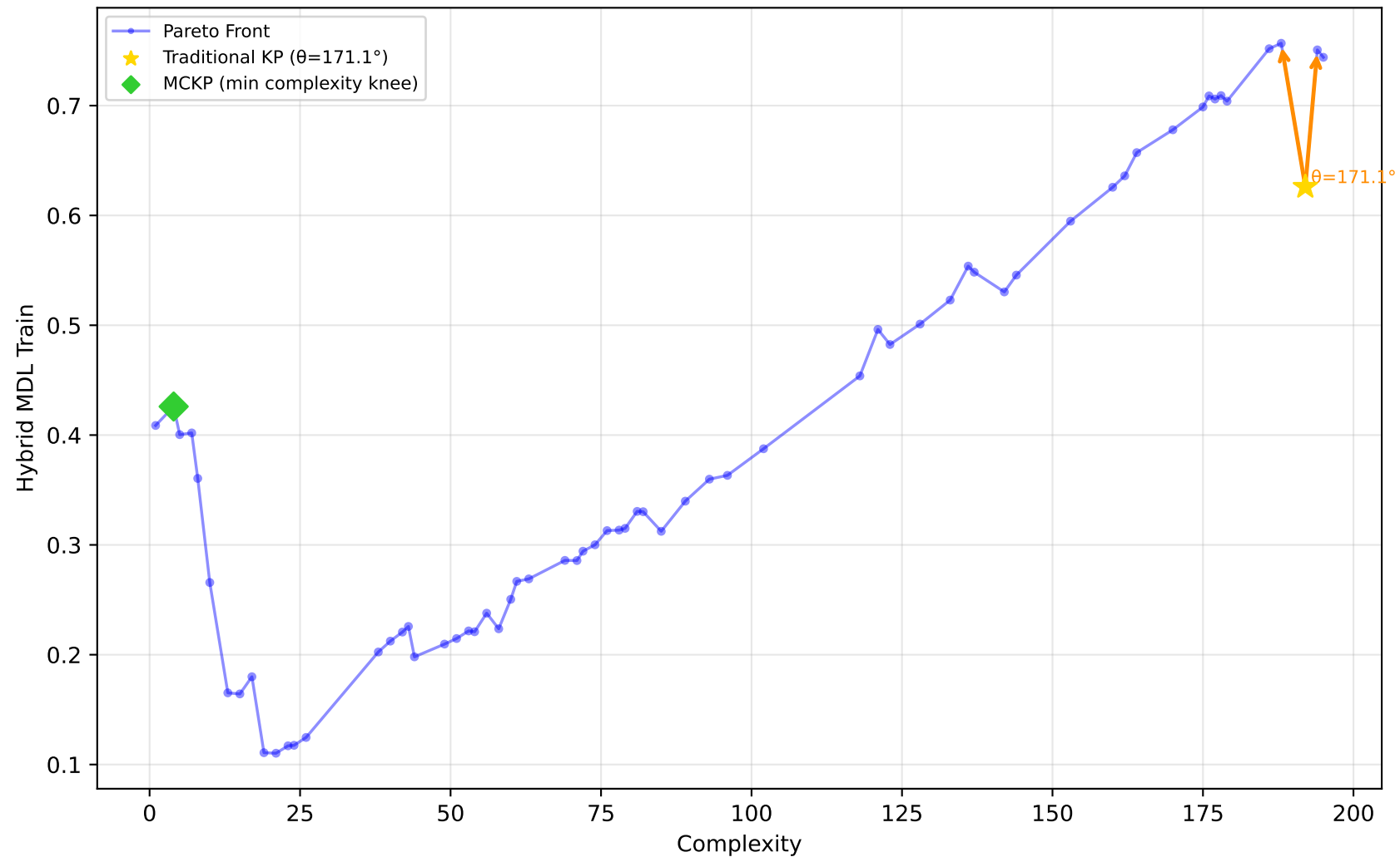
556_analcatdata_apnea2 - Run 5 - MVP - Hybrid MDL Train \lambda_1=0.00, \lambda_2=0.00, \lambda_3=0.00 | Difficulty: 1.00 | Method: hmr
