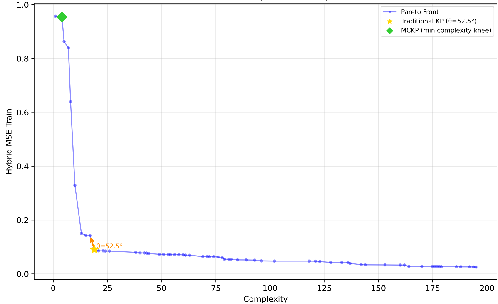
556_analcatdata_apnea2 - Run 5 - MVP - Hybrid MSE Train \lambda_1=0.00, \lambda_2=0.00, \lambda_3=0.00 | Difficulty: 1.00 | Method: hmr
