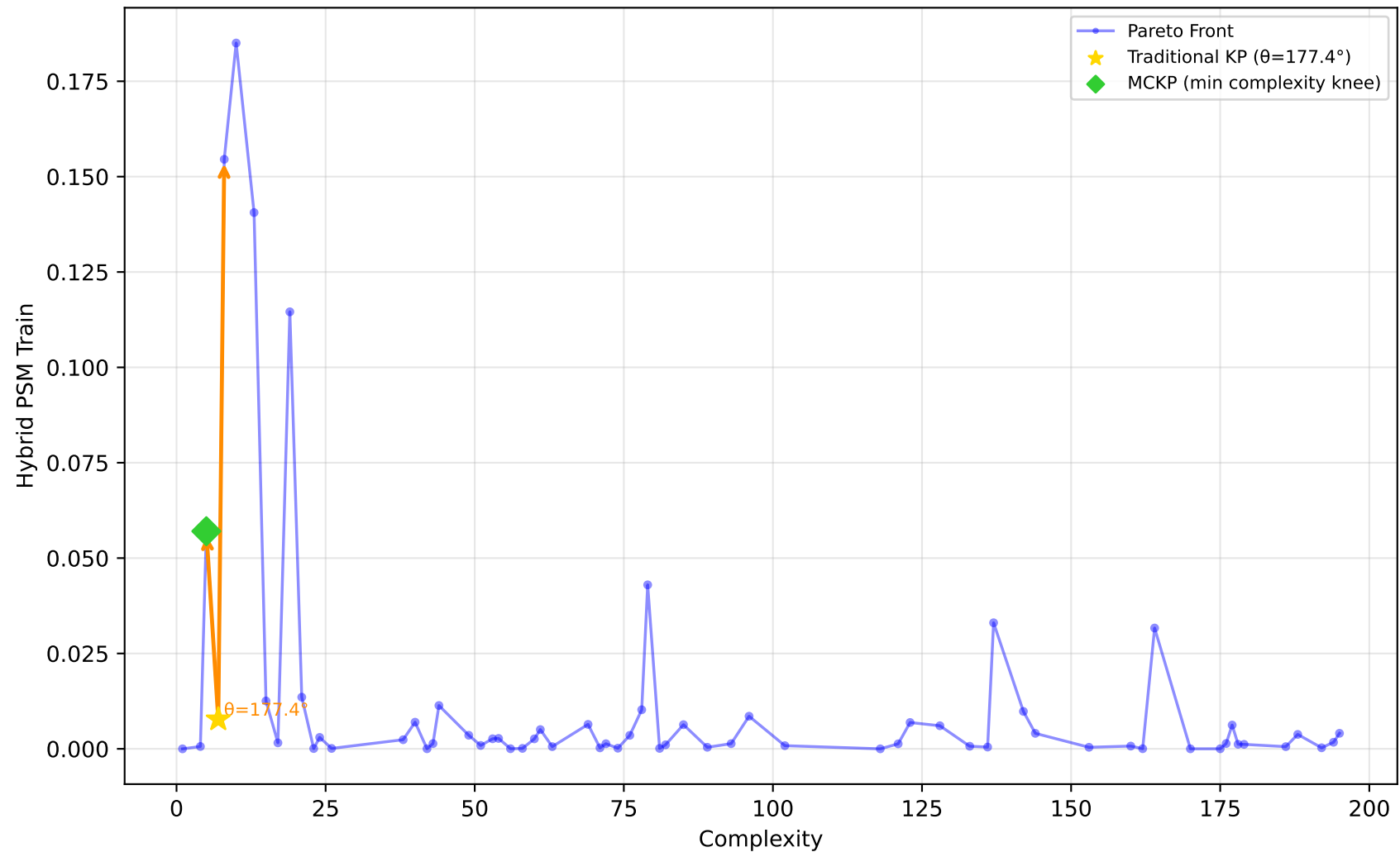
556_analcatdata_apnea2 - Run 5 - MVP - Hybrid PSM Train \lambda_1=0.00, \lambda_2=0.00, \lambda_3=0.00 | Difficulty: 1.00 | Method: hmr
