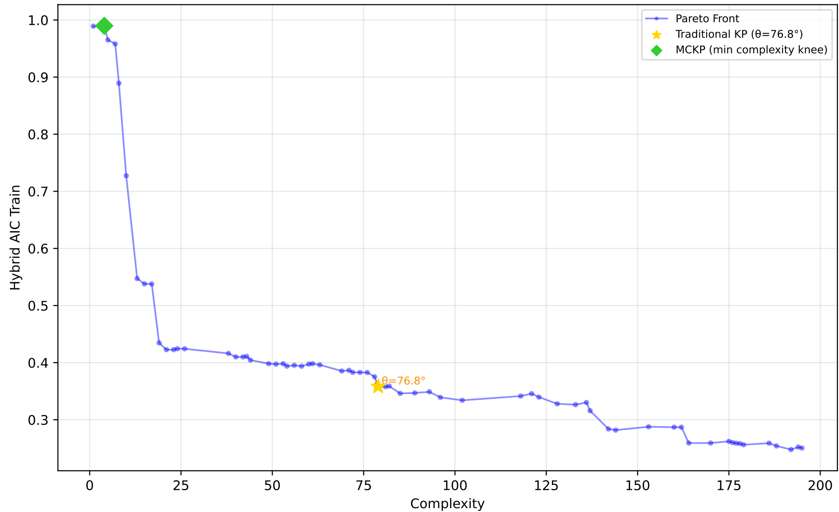
556_analcatdata_apnea2 - Run 5 - SVP - Hybrid AIC Train \lambda_1=0.00, \lambda_2=0.00, \lambda_3=0.00 | Difficulty: 1.00 | Method: hmr
