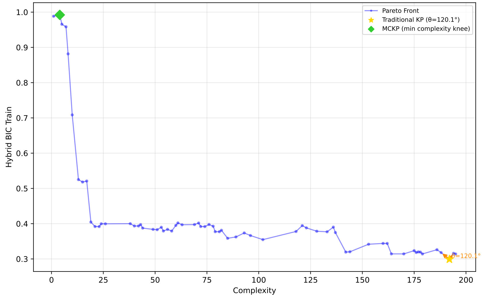
556_analcatdata_apnea2 - Run 5 - SVP - Hybrid BIC Train \lambda_1=0.00 , \lambda_2=0.00 , \lambda_3=0.00 | Difficulty: 1.00 | Method: hmr
