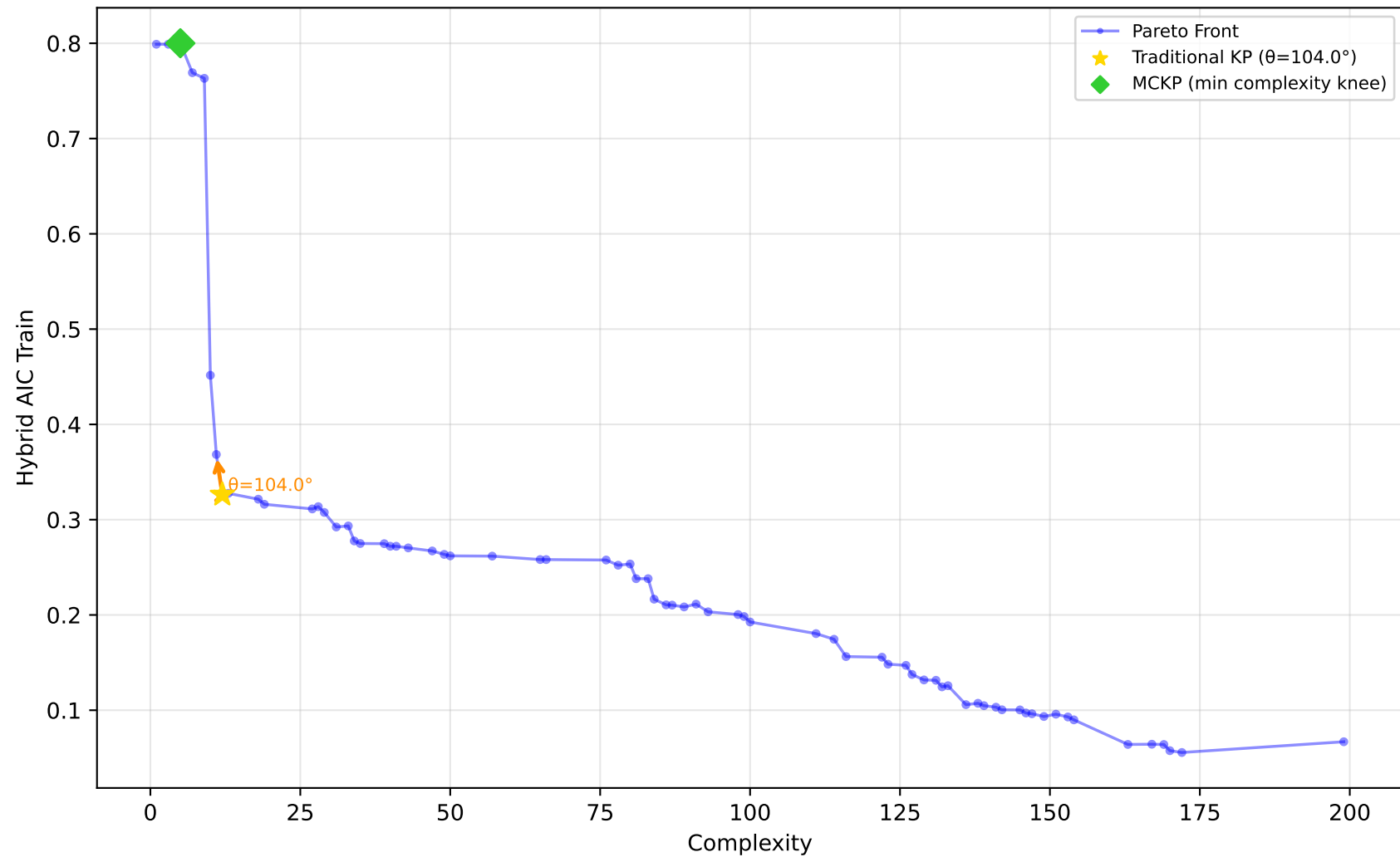
556_analcatdata_apnea2 - Run 6 - MVP - Hybrid AIC Train \lambda_1=0.00, \lambda_2=0.00, \lambda_3=0.00 | Difficulty: 0.83 | Method: hmr
