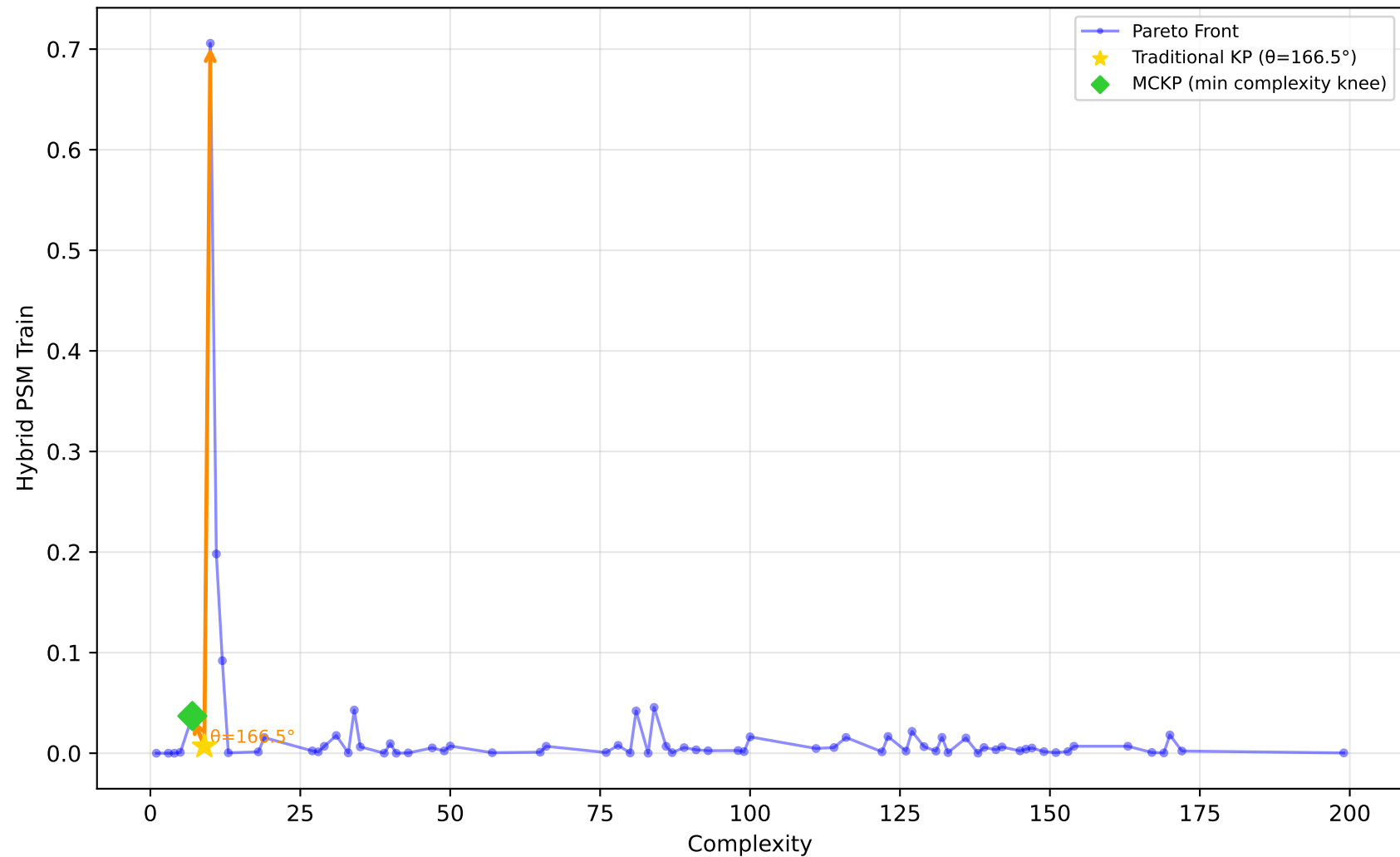
556_analcatdata_apnea2 - Run 6 - MVP - Hybrid PSM Train \lambda_1=0.00, \lambda_2=0.00, \lambda_3=0.00 | Difficulty: 0.83 | Method: hmr
