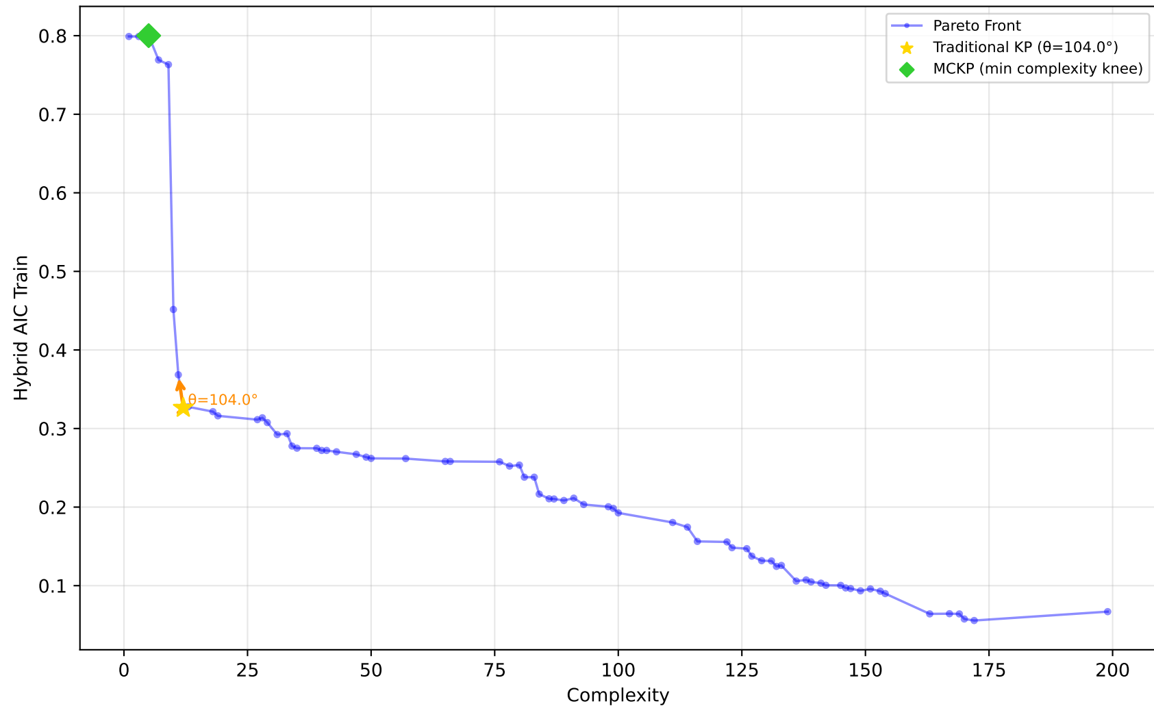
556_analcatdata_apnea2 - Run 6 - SVP - Hybrid AIC Train \lambda_1=0.00, \lambda_2=0.00, \lambda_3=0.00 | Difficulty: 0.83 | Method: hmr
