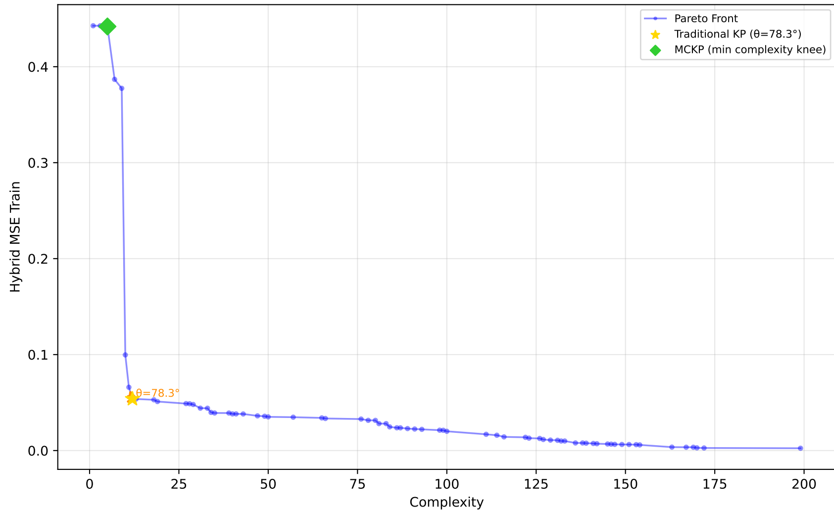
556_analcatdata_apnea2 - Run 6 - SVP - Hybrid MSE Train \lambda_1=0.00, \lambda_2=0.00, \lambda_3=0.00 | Difficulty: 0.83 | Method: hmr
