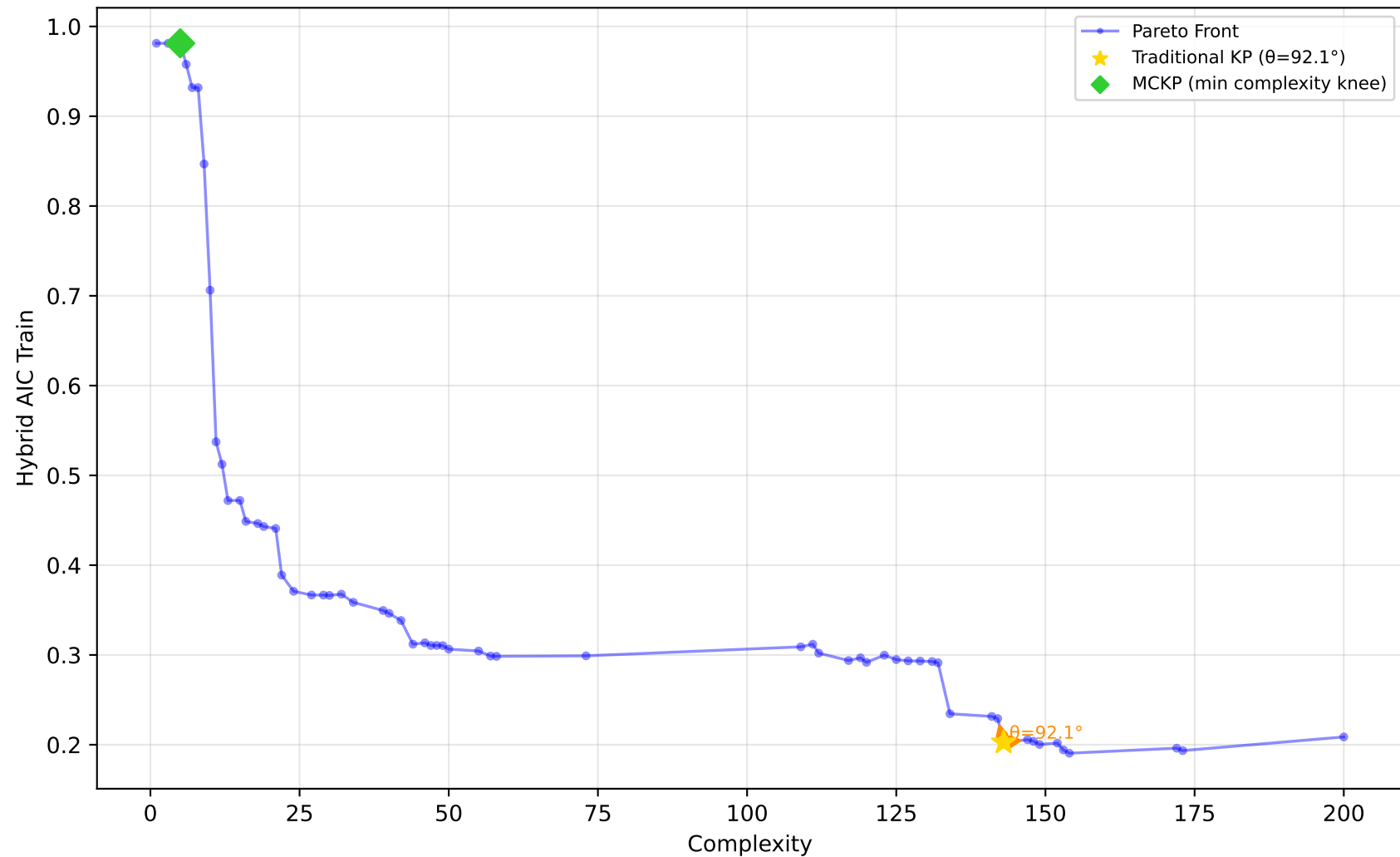
556_analcatdata_apnea2 - Run 7 - MVP - Hybrid AIC Train \lambda_1=0.00, \lambda_2=0.00, \lambda_3=0.00 | Difficulty: 1.00 | Method: hmr
