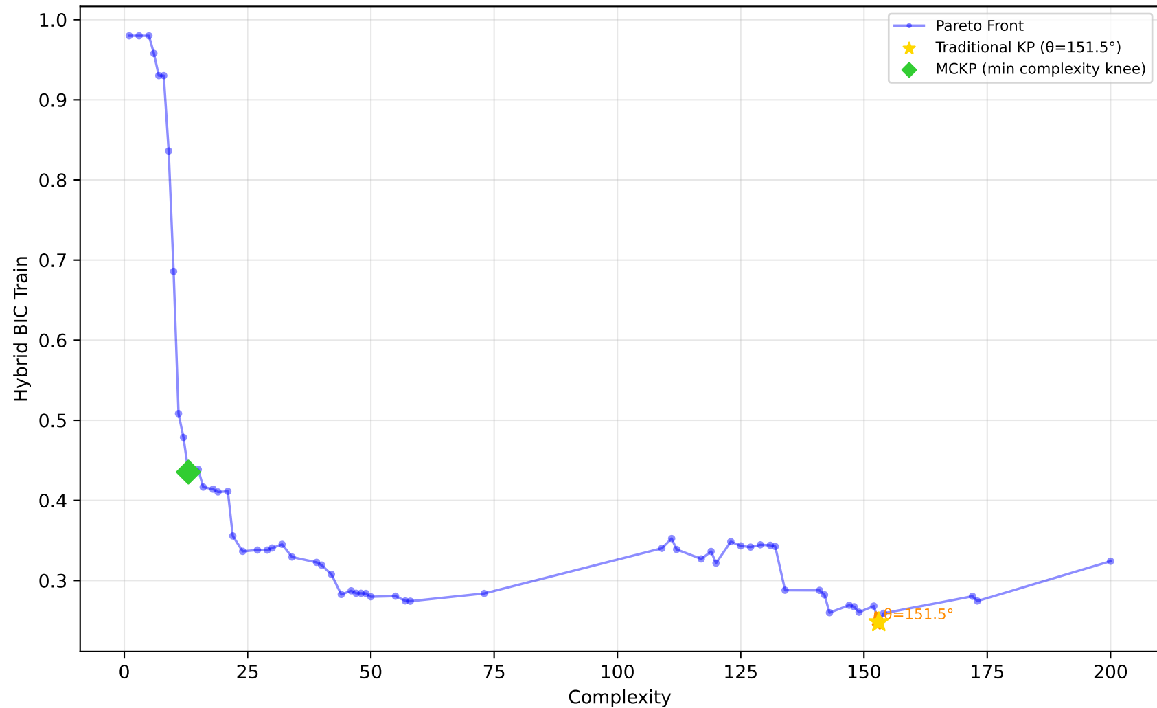
556_analcatdata_apnea2 - Run 7 - MVP - Hybrid BIC Train \lambda_1=0.00, \lambda_2=0.00, \lambda_3=0.00 | Difficulty: 1.00 | Method: hmr
