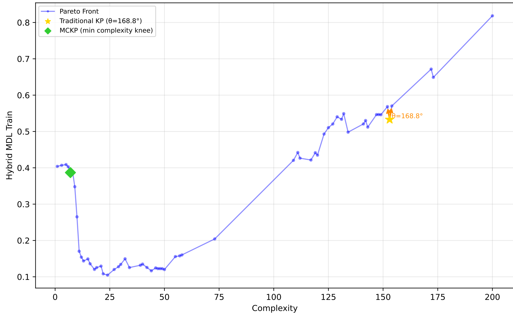
556_analcatdata_apnea2 - Run 7 - MVP - Hybrid MDL Train \lambda_1=0.00, \lambda_2=0.00, \lambda_3=0.00 | Difficulty: 1.00 | Method: hmr
