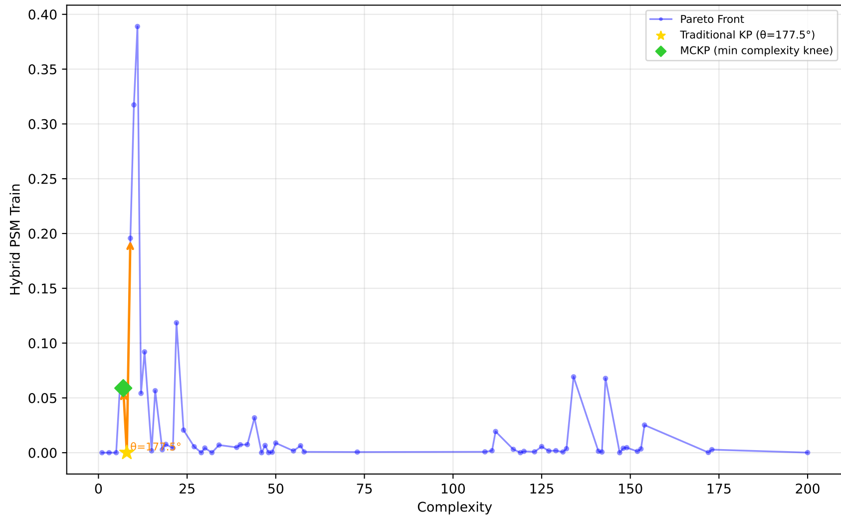
556_analcatdata_apnea2 - Run 7 - MVP - Hybrid PSM Train \lambda_1=0.00 , \lambda_2=0.00 , \lambda_3=0.00 | Difficulty: 1.00 | Method: hmr
