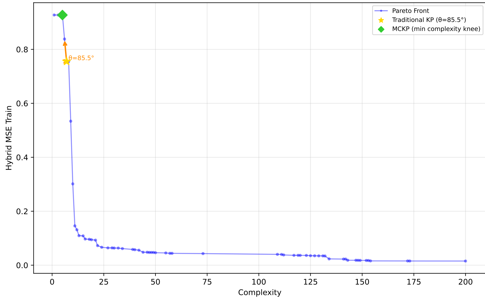
556_analcatdata_apnea2 - Run 7 - SVP - Hybrid MSE Train \lambda_1=0.00, \lambda_2=0.00, \lambda_3=0.00 | Difficulty: 1.00 | Method: hmr
