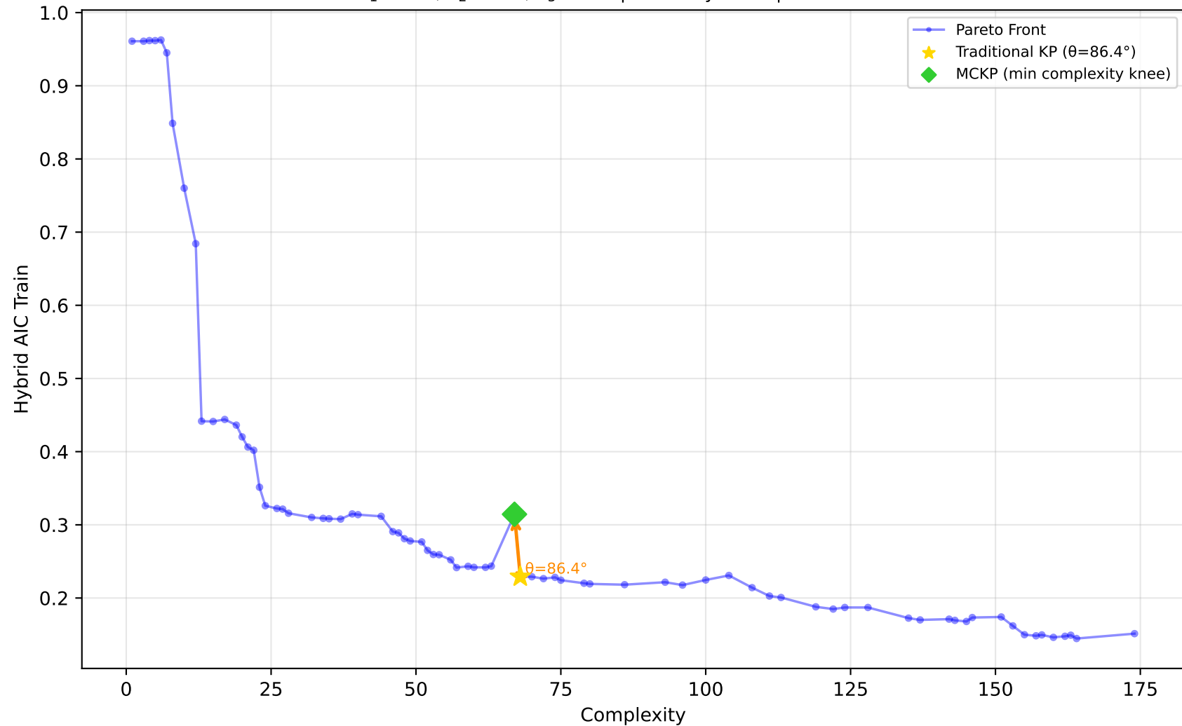
556_analcatdata_apnea2 - Run 8 - MVP - Hybrid AIC Train \lambda_1=0.00, \lambda_2=0.00, \lambda_3=0.00 | Difficulty: 1.00 | Method: hmr
