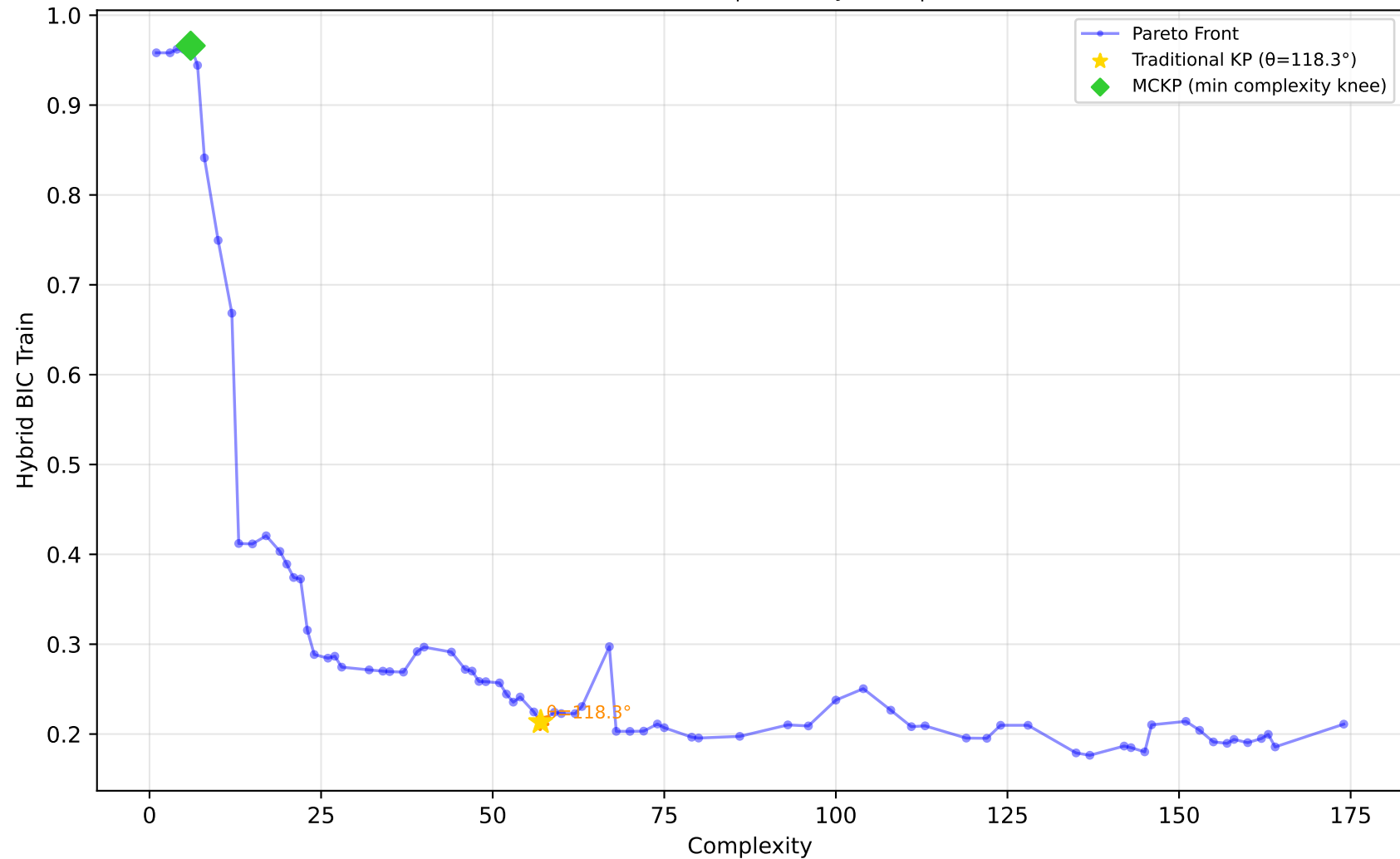
556_analcatdata_apnea2 - Run 8 - MVP - Hybrid BIC Train \lambda_1=0.00, \lambda_2=0.00, \lambda_3=0.00 | Difficulty: 1.00 | Method: hmr
