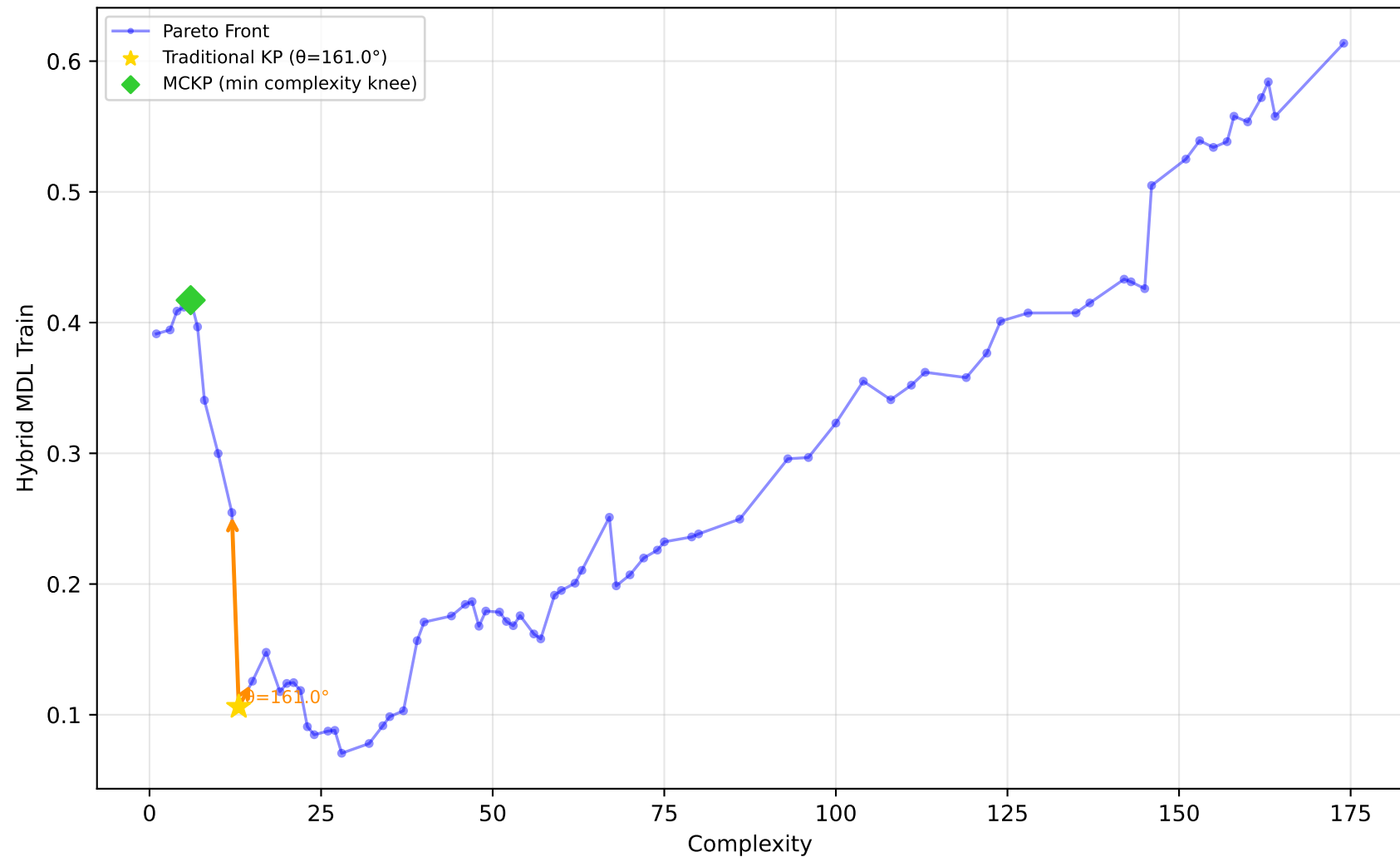
556_analcatdata_apnea2 - Run 8 - MVP - Hybrid MDL Train \lambda_1=0.00, \lambda_2=0.00, \lambda_3=0.00 | Difficulty: 1.00 | Method: hmr
