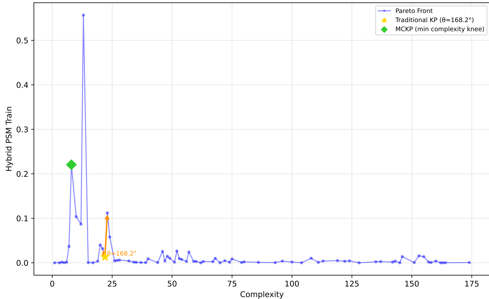
556_analcatdata_apnea2 - Run 8 - MVP - Hybrid PSM Train \lambda_1=0.00, \lambda_2=0.00, \lambda_3=0.00 | Difficulty: 1.00 | Method: hmr
