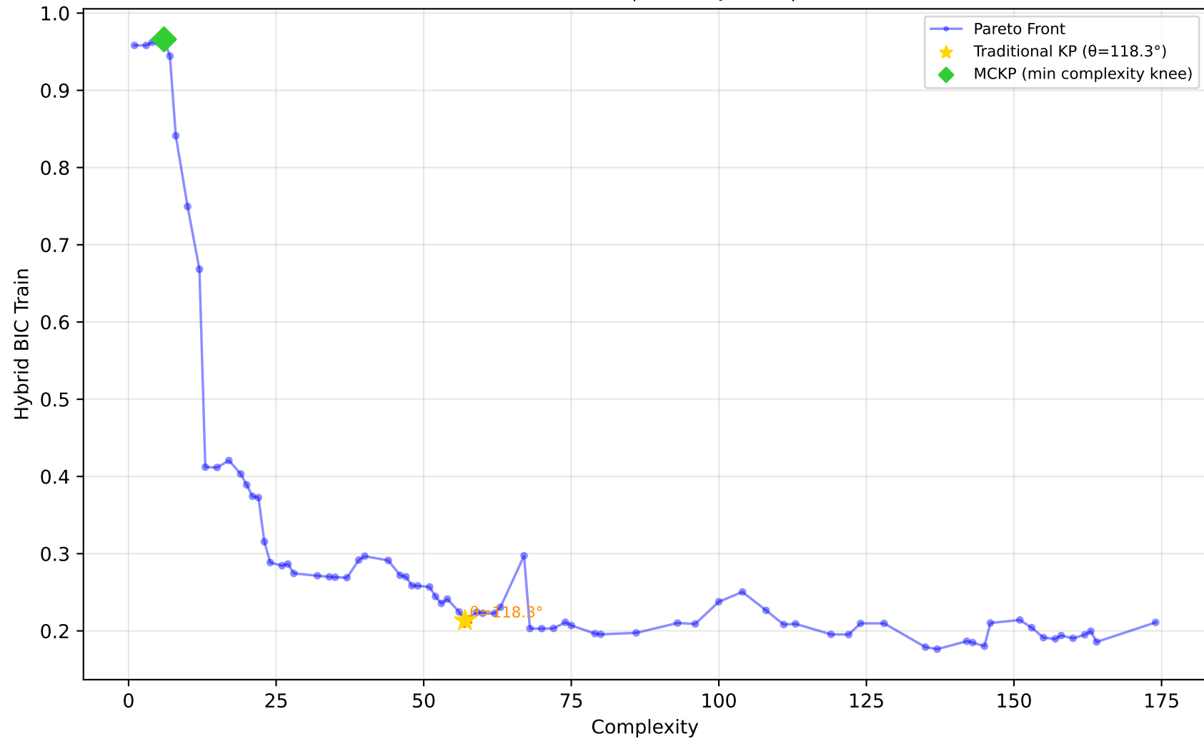
556_analcatdata_apnea2 - Run 8 - SVP - Hybrid BIC Train \lambda_1=0.00, \lambda_2=0.00, \lambda_3=0.00 | Difficulty: 1.00 | Method: hmr
