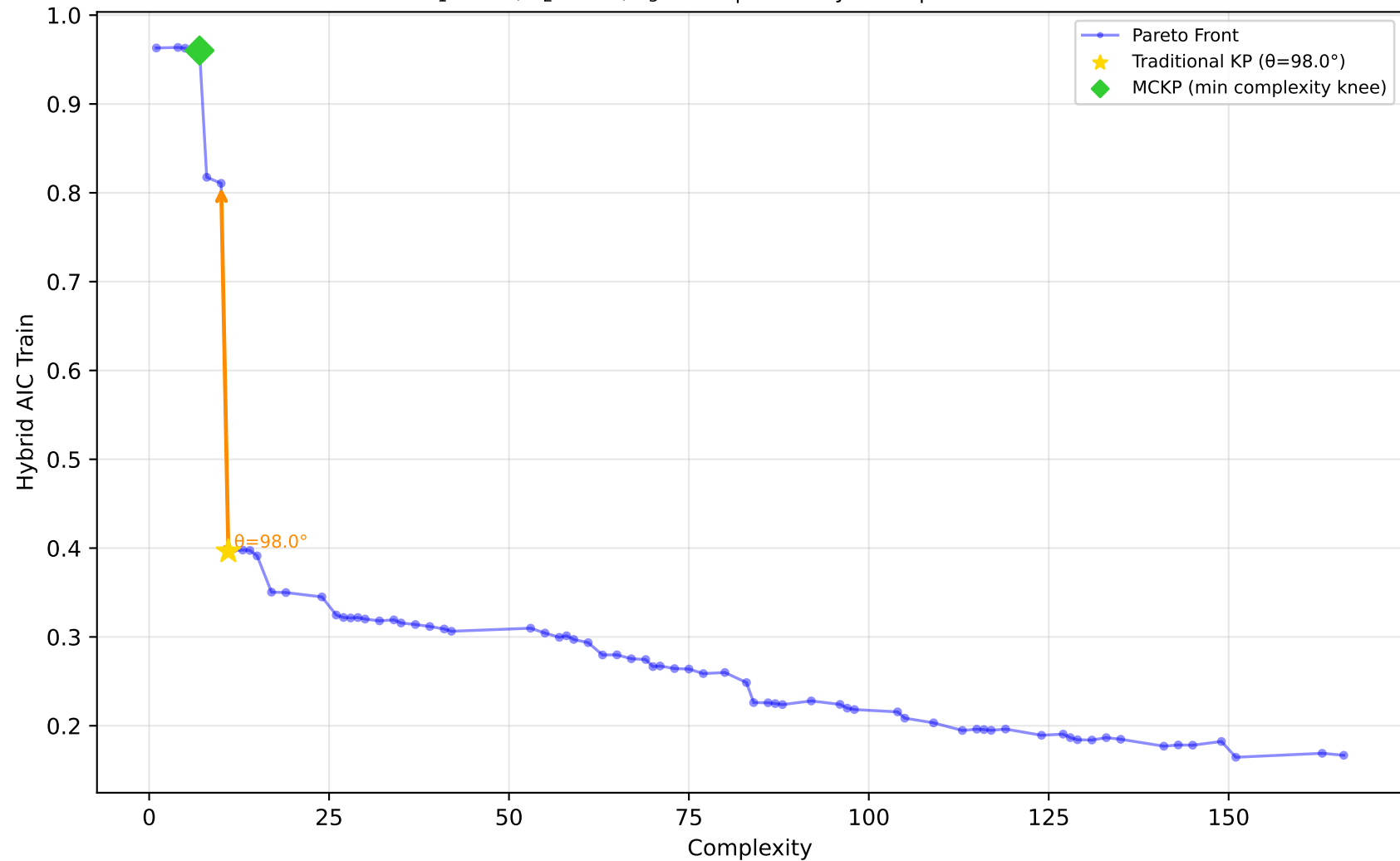
556_analcatdata_apnea2 - Run 9 - MVP - Hybrid AIC Train \lambda_1=0.00, \lambda_2=0.00, \lambda_3=0.00 | Difficulty: 0.82 | Method: hmr
